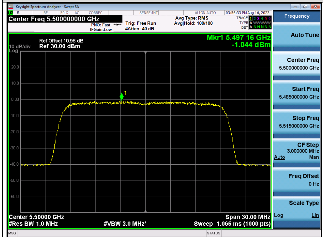
Test_Graph_802.11ax20_ANT1_5500_MCS0_PSD
