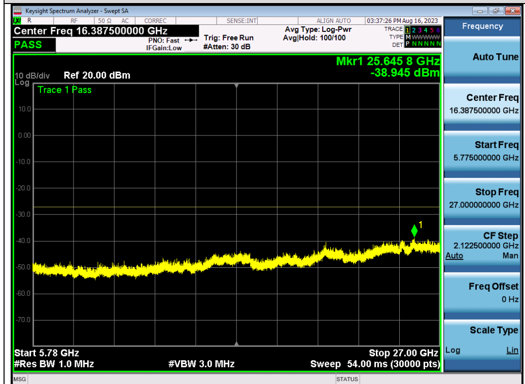
Test_Graph_802.11n40_ANT1_5670_MCS0_Frequency Band 4
