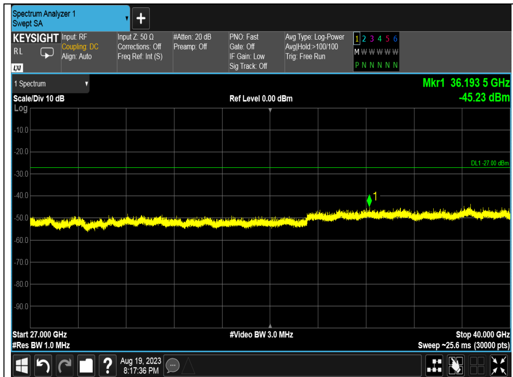
Test_Graph_802.11a_ANT2_5700_6Mbps_Frequency Band 5
