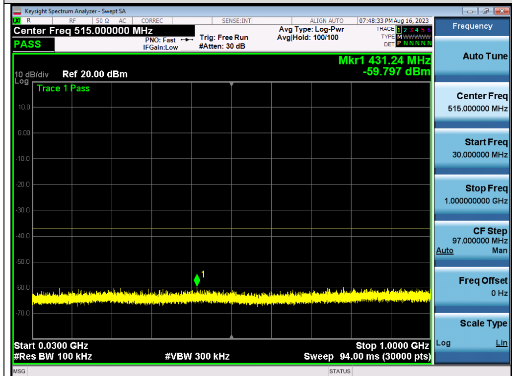
Test_Graph_802.11n40_ANT2_5510_MCS0_Frequency Band 1
