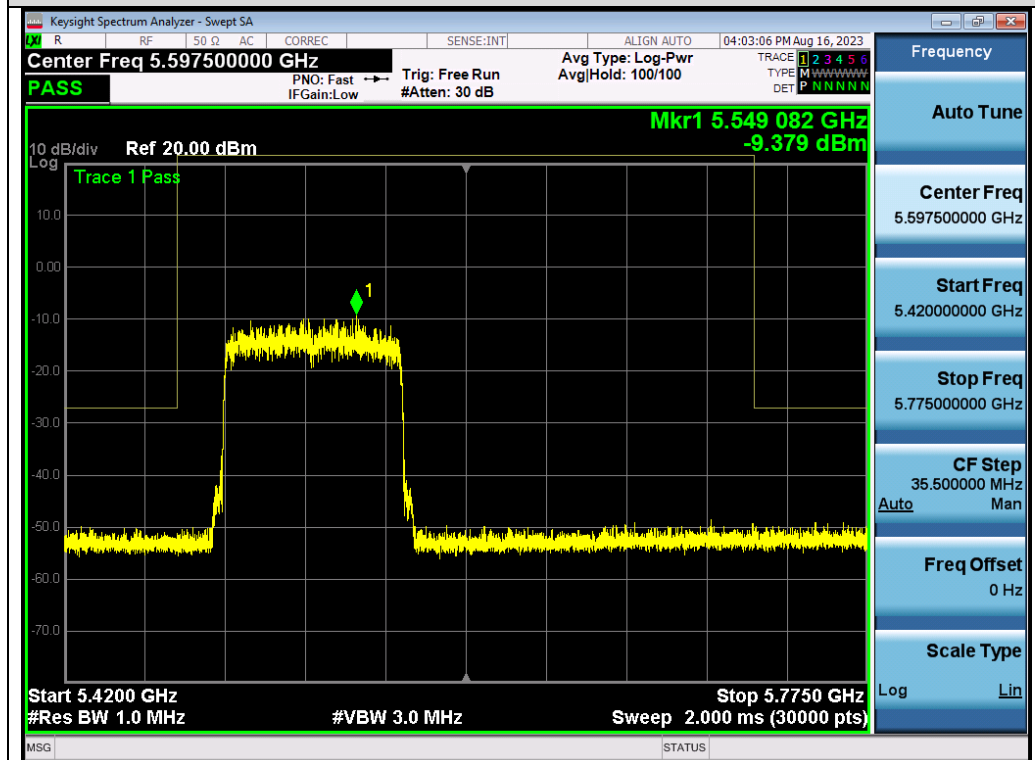
Test_Graph_802.11ax80_ANT1_5530_MCS9_Frequency Band 3
