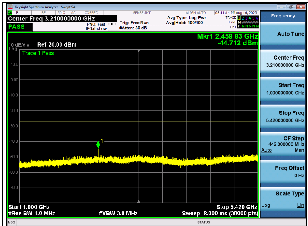
Test_Graph_802.11ac80_ANT2_5610_MCS9_Frequency Band 2
