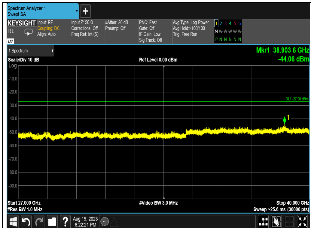
Test_Graph_802.11ax80_ANT2_5530_MCS9_Frequency Band 5
