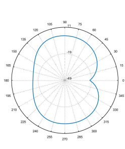
Total_Polar_E1_5.15GHz
