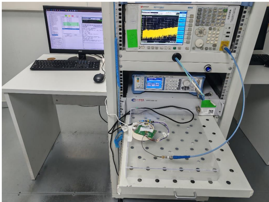
Conducted Test- BLE/2.4G WIFI
