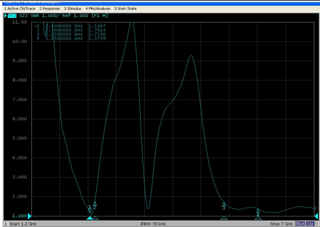
2.4+5.8G WIFI antenna VSWR
