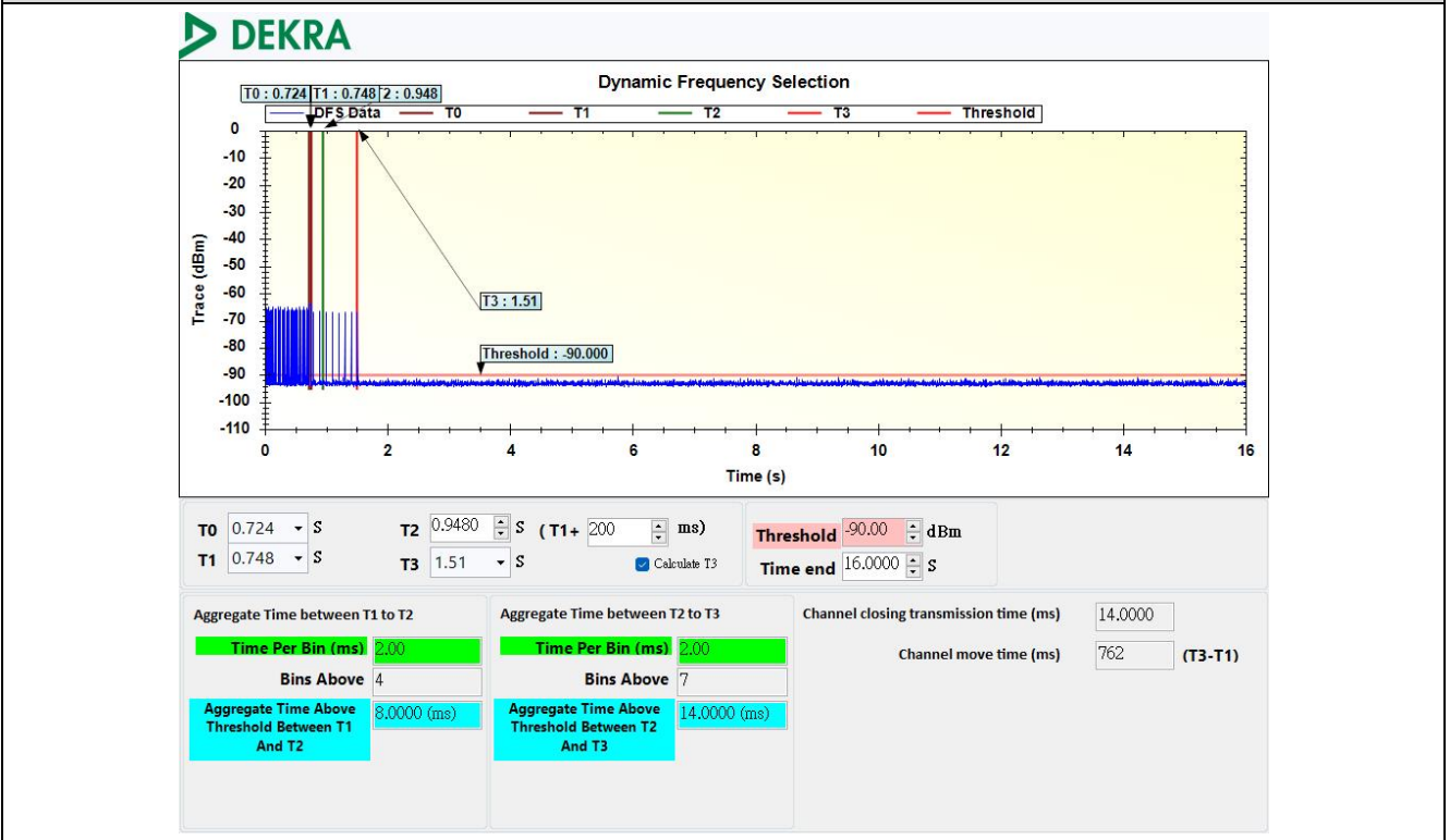
Channel Move Time and Channel Closing Transmission Time - 802.11ac (80 MHz), 5530 MHz
