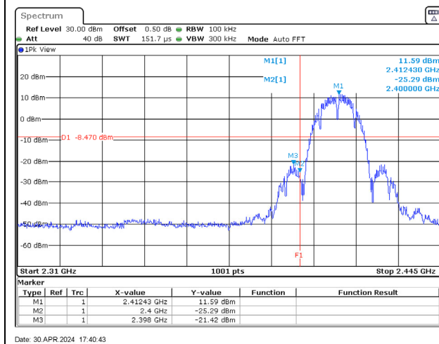
802.11g / 2412 MHz
