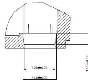
Detail A (10/1)
