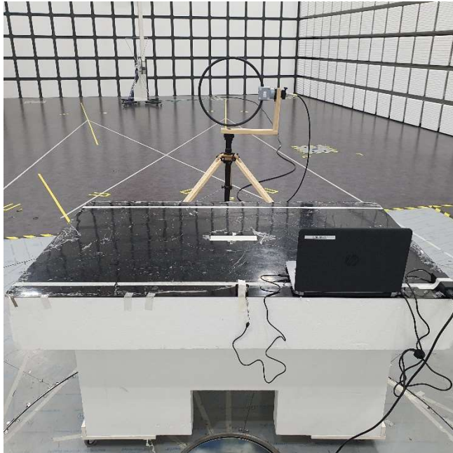
BELOW 30 MHz REAR TEST PHOTO
