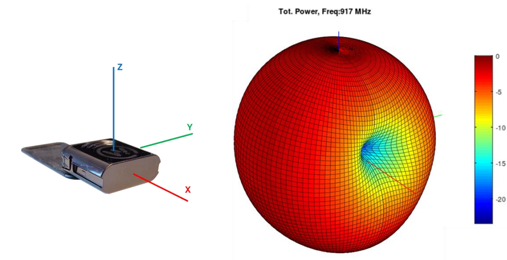
Figure 4-4 3D- radiation pattern @917MHz. Wittra CXAMELEON-1.0-US 915MHz antenna.
