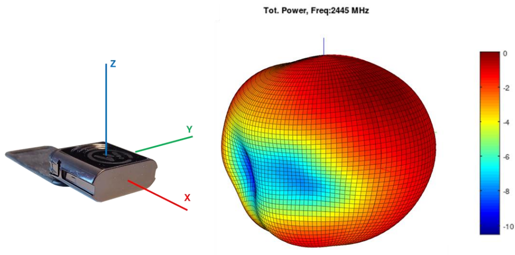
Figure 4-5 3D- radiation pattern @2445MHz. Wittra CXAMELEON-1.0-US 2400MHz antenna.
