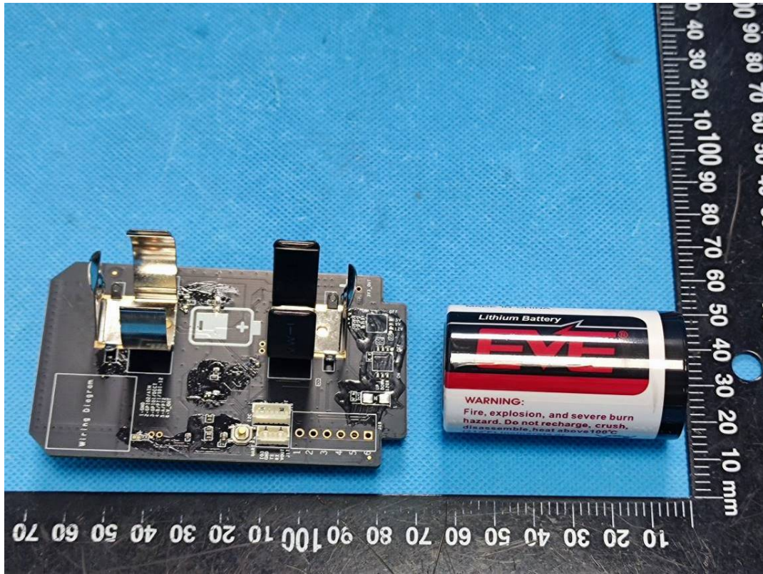
Battery 1#
