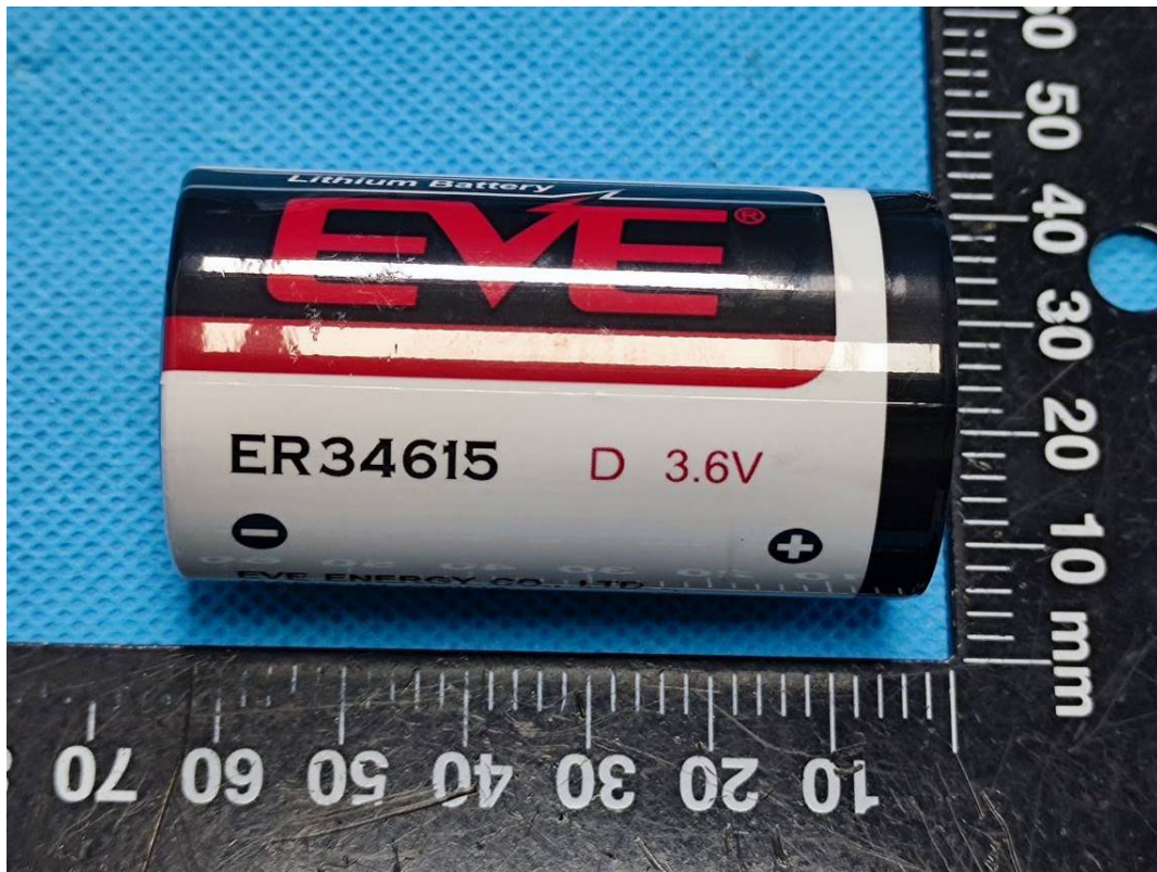
Battery 1#
