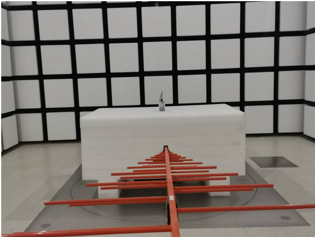
Radiated Emission Below 1GHz View- EM500-PP-915M
