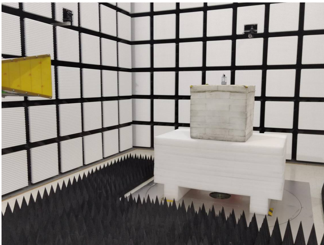
Radiated Emission Above 1GHz View EM500-LGT-915M
