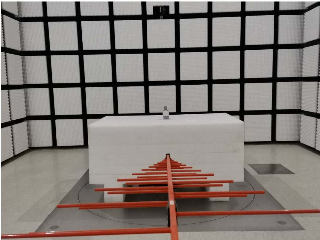
Radiated Emission Below 1GHz View- EM500-CO2-915M
