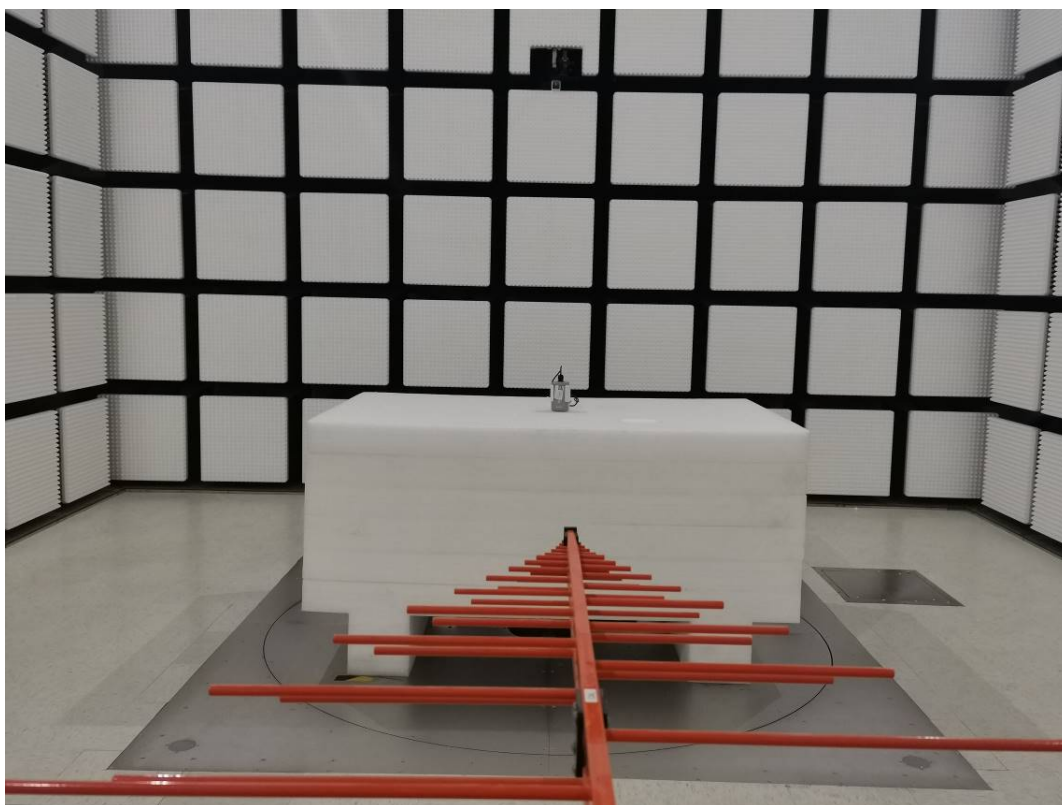
Radiated Emission Below 1GHz View- EM500-SMT-915M
