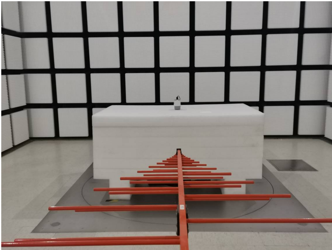
Radiated Emission Below 1GHz View- EM500-LGT-915M
