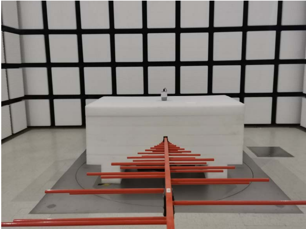
Radiated Emission Above 1GHz View EM500-LGT-915M
