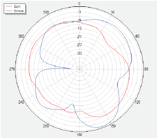
Phi=0 freq=2400MHz
