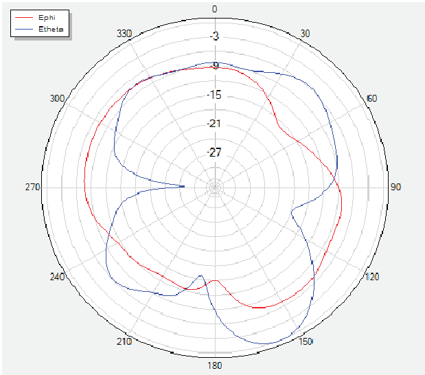
Phi=0 freq=2500MHz
