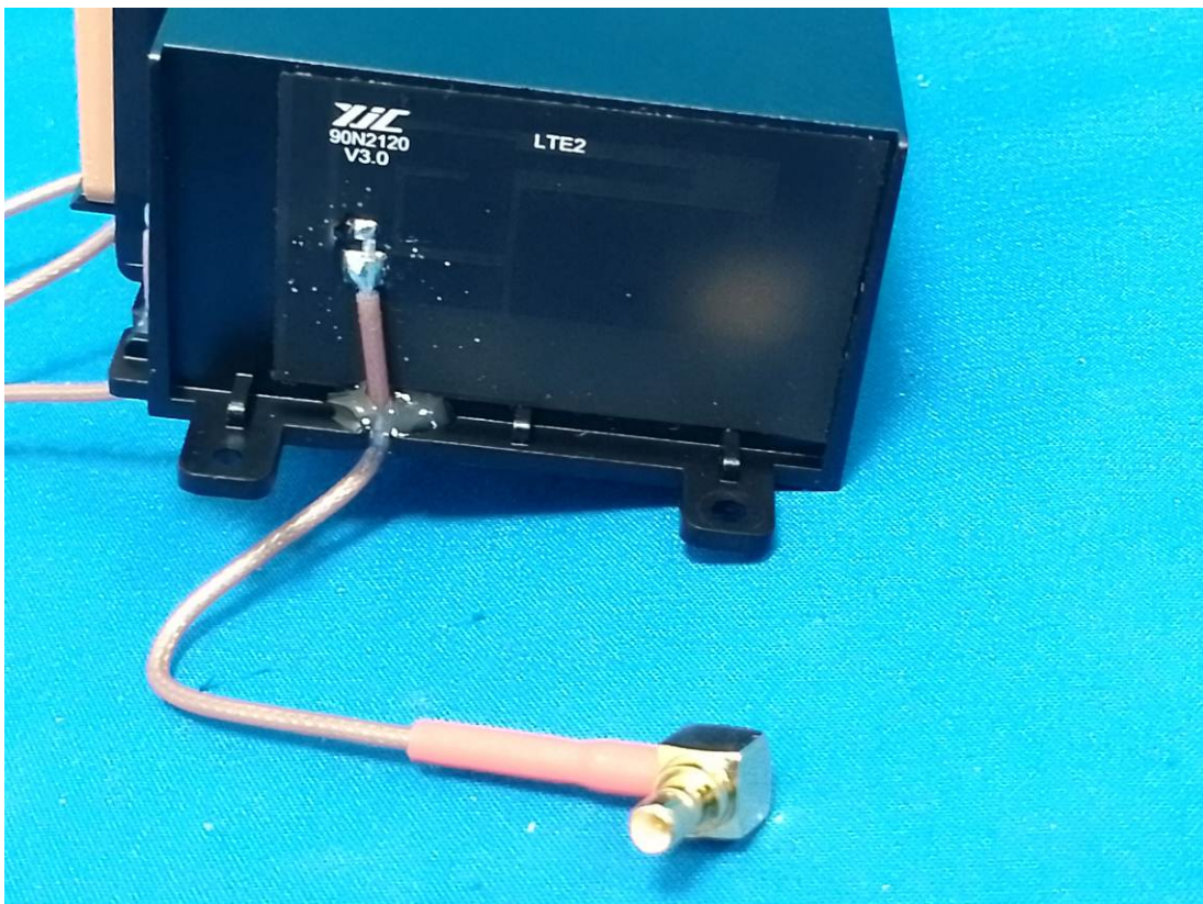
WWAN Antenna(LTE 2): only receive
