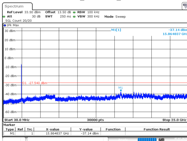
802.11n40_2452MHz_Chain 1
