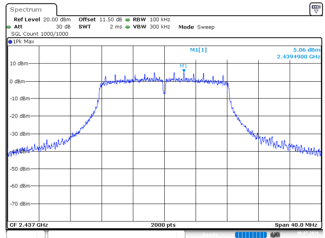
802.11g_2437MHz_Chain 0
