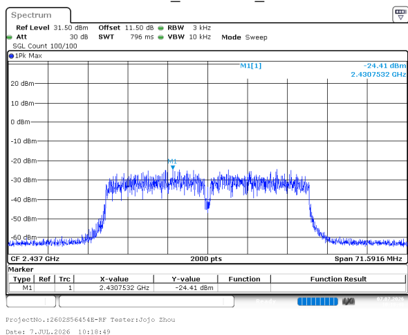
802.11n40_2437MHz_Chain 1
