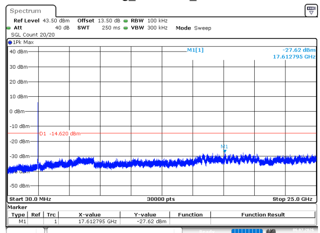
802.11g_2462MHz_Chain 0
