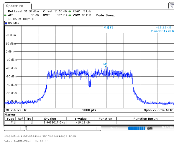
802.11n40_2437MHz_Chain 0
