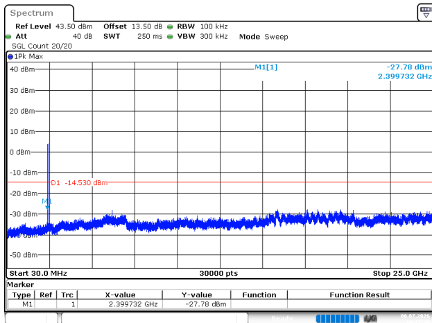
802.11g_2412MHz_Chain 0
