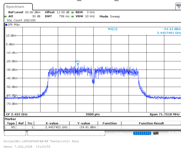
802.11n40_2452MHz_Chain 1
