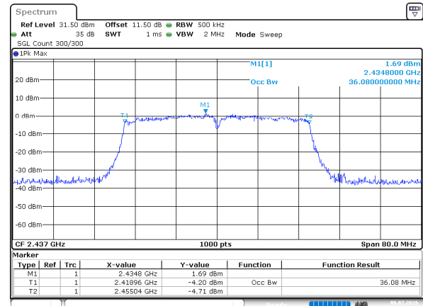
802.11n40_2437MHz_Chain 0
