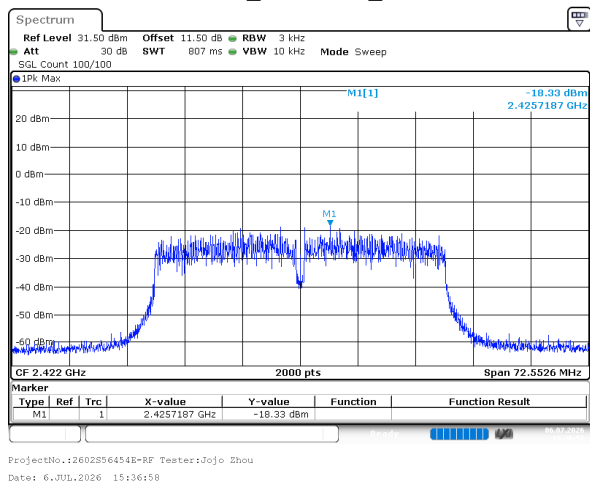
802.11n40_2422MHz_Chain 0
