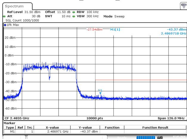
802.11n40_2452MHz_Chain 1
