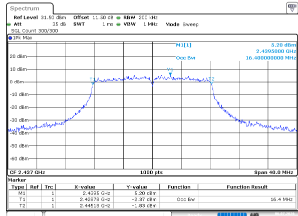
802.11g_2437MHz_Chain 0
