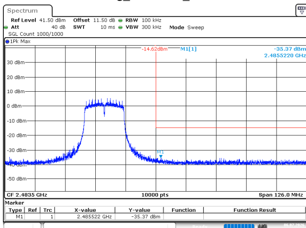
802.11g_2462MHz_Chain 0
