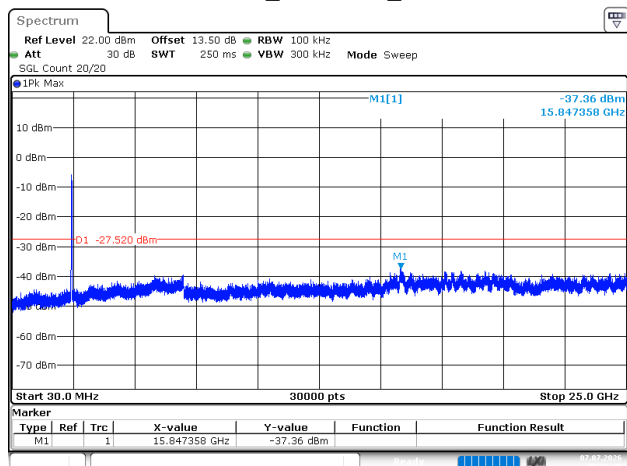
802.11n40_2437MHz_Chain 1
