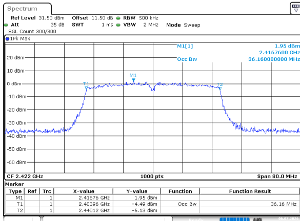
802.11n40_2422MHz_Chain 0
