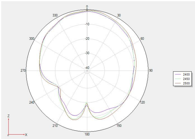
Phi 0 2D
