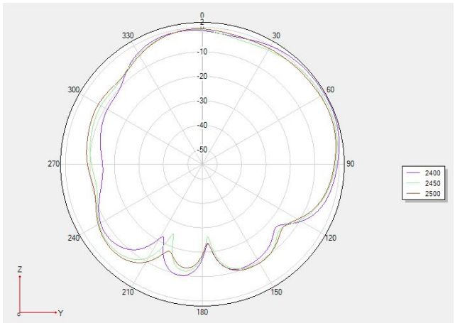
Phi 90 2D
