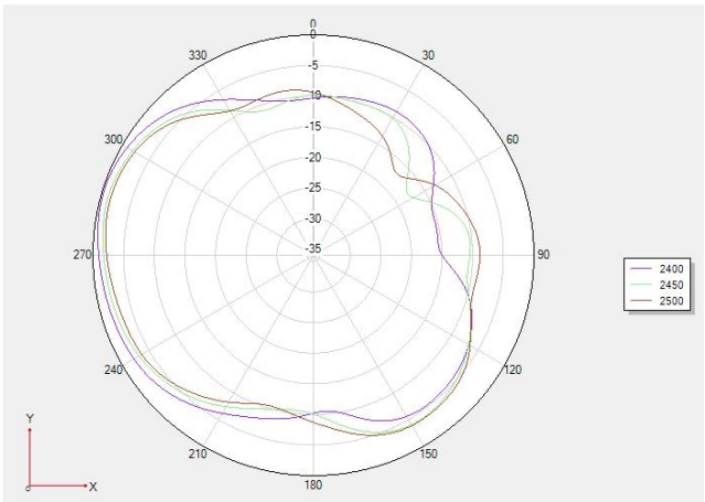
Theta 90 2D
