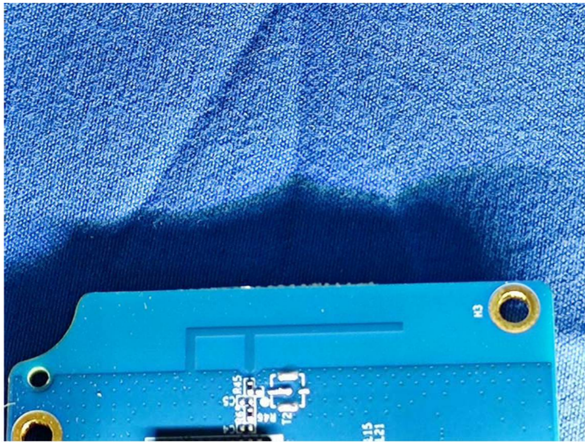
WIFI Antenna
