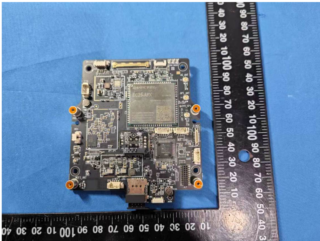
Contain WWAN module, FCC ID:XMR201909EC25AFX
