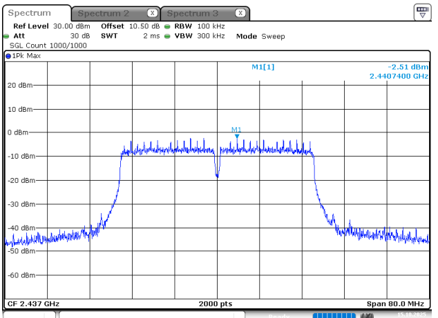
802.11n40_2437MHz
