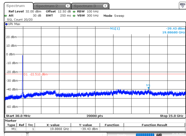
802.11n40_2437MHz
