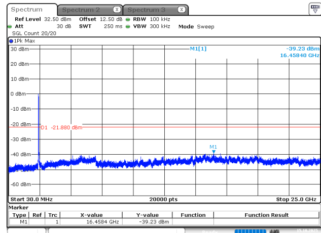
802.11n40_2422MHz
