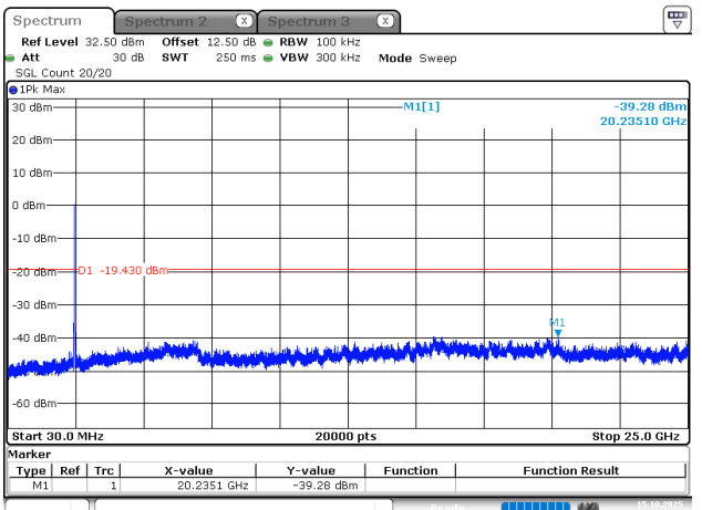
802.11g_2462MHz
