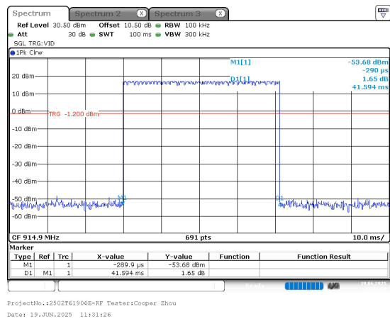
Pulse width=41.594ms
