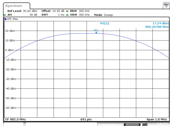
Low Channel
