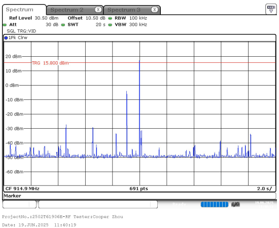
Observation time=20s
