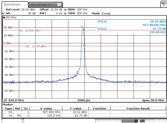
High_Single
