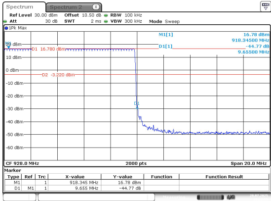
High_Hopping
