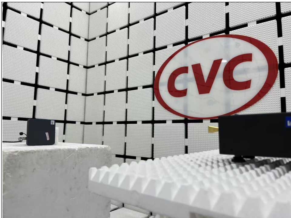
RADIATED EMISSION TEST (40GHz ~ 100GHz)
