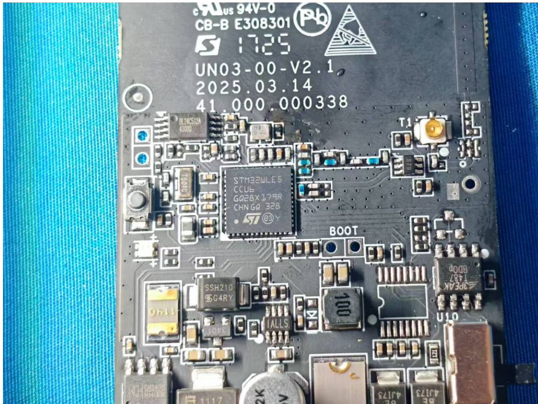
Lora Antenna(no use)
