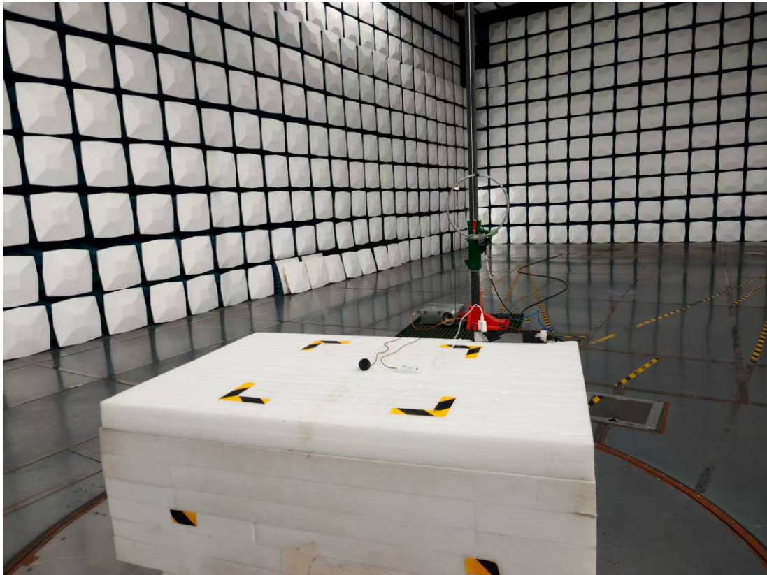
Radiated Emission 9k-30MHz Perpendicular View Chain 1
