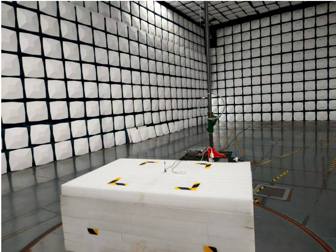
Radiated Emission 9k-30MHz Perpendicular View Chain 0
