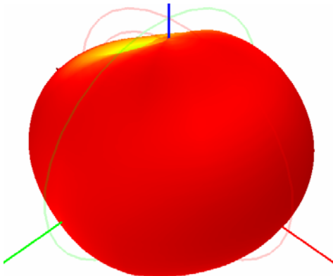
915.0MHz H+V, Eff: 48.9%
