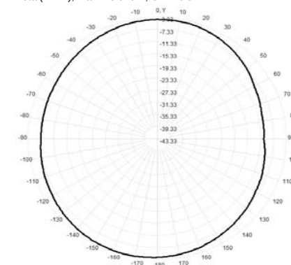
Total(H-XY), Max= -3.94dBi, CirD=6.57
