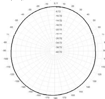
Total(H-XY), Max= -3.26dBi, CirD=5.75
