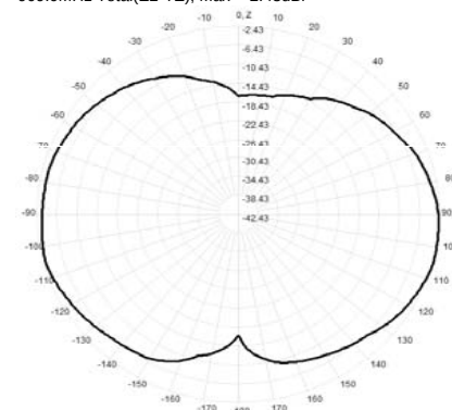
909.0MHz Total(E2-YZ), Max= -2.43dBi
