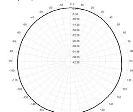
Total(H-XY), Max= -2.75dBi, CirD=4.76
