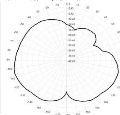
909.0MHz Total(E1-XZ), Max= -4.45dBi
