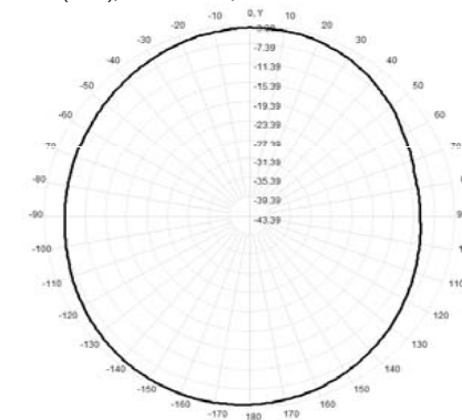
Total(H-XY), Max= -4.00dBi, CirD=6.33
