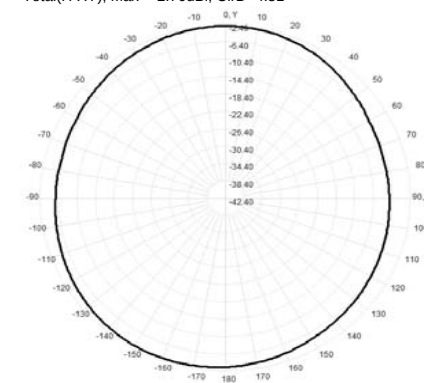
Total(H-XY), Max= -2.77dBi, CirD=4.70
