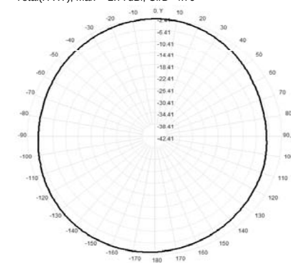
Total(H-XY), Max= -2.75dBi, CirD=4.76
