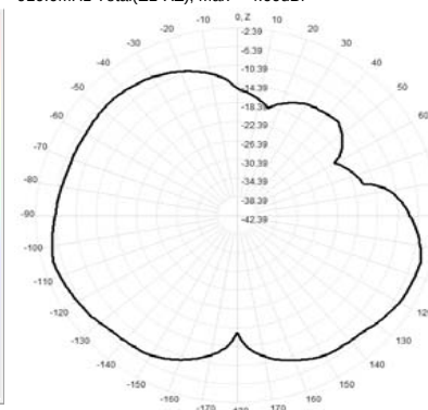
910.0MHz Total(E1-XZ), Max= -4.60dBi
