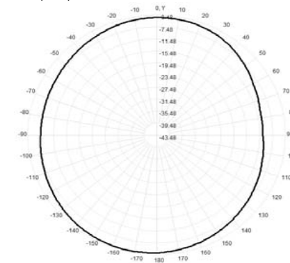
Total(H-XY), Max= -4.12dBi, CirD=6.55
