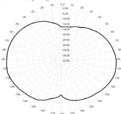
914.0MHz Total(E2-YZ), Max= -2.59dBi
