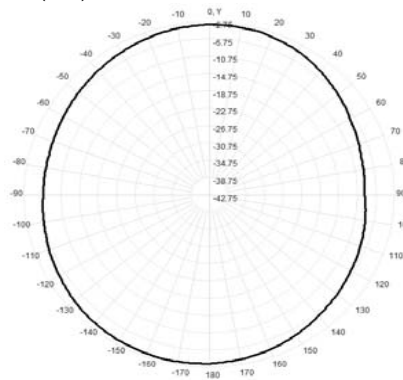
Total(H-XY), Max= -3.41dBi, CirD=5.96
