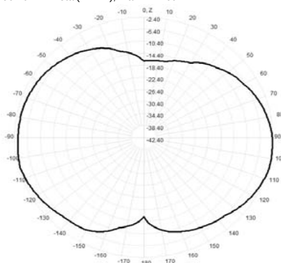
907.0MHz Total(E2-YZ), Max= -2.40dBi
