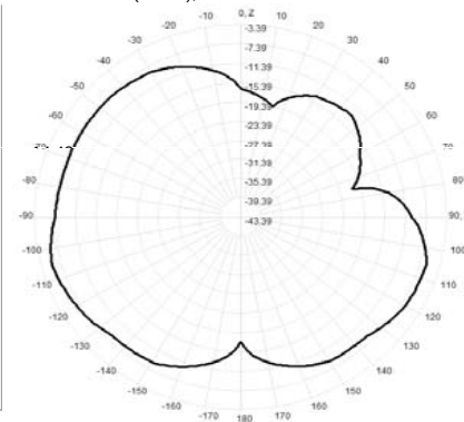
924.0MHz Total(E1-XZ), Max= -5.52dBi
