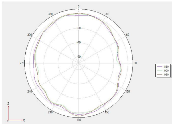
Phi 0 2D
