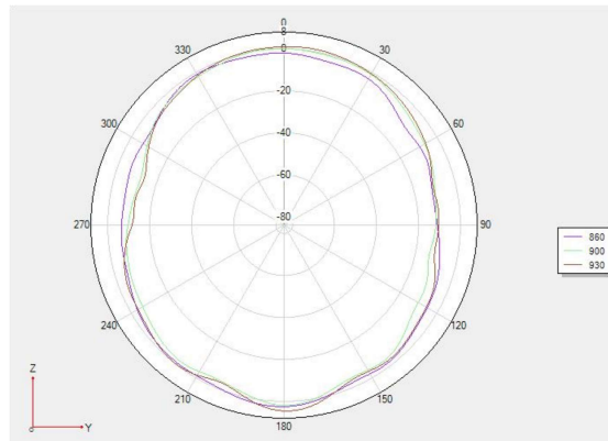
Phi 90 2D
