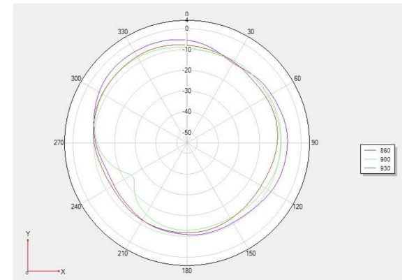
Theta 90 2D
