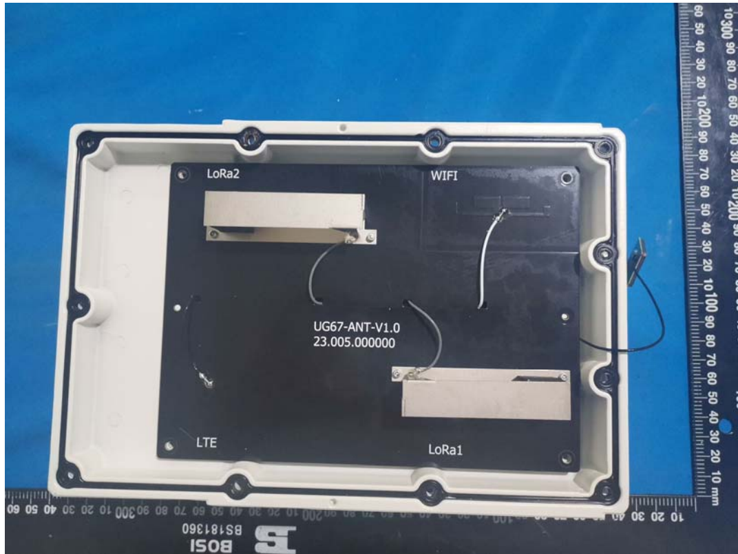
Antenna Board
