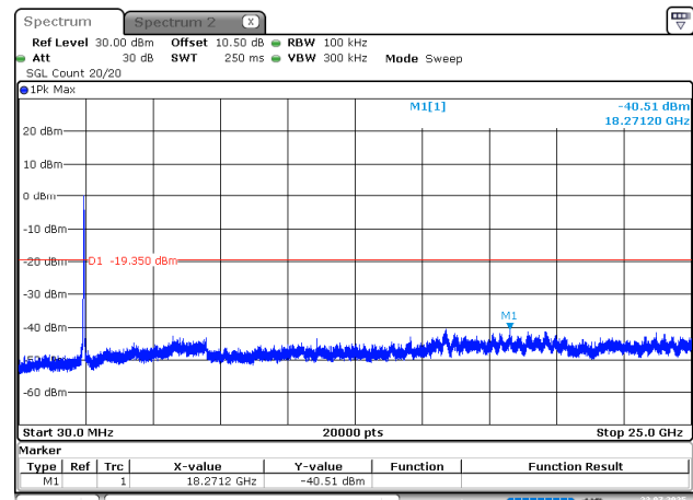
802.11n40_2437MHz
