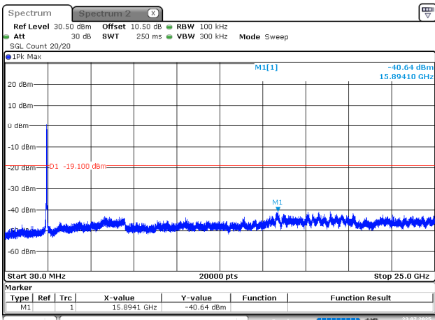
802.11n40_2452MHz
