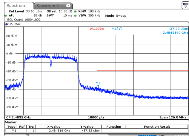
802.11n40_2452MHz
