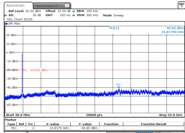
802.11n40_2422MHz
