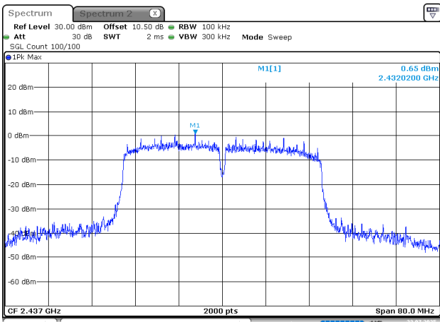
802.11n40_2437MHz
