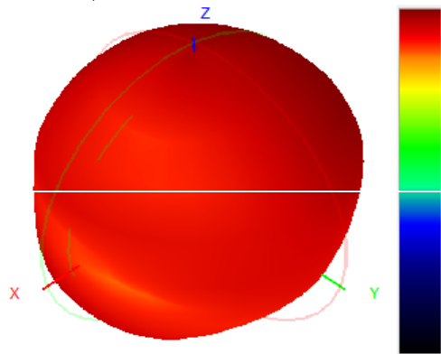
924.0MHz H+V, Eff: 22.0%
