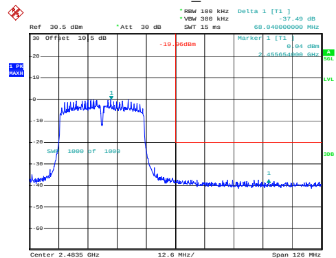
802.11n40_2452MHz
