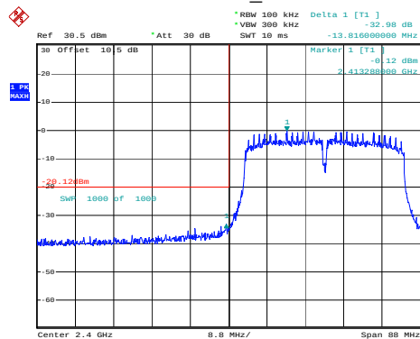
802.11n40_2422MHz
