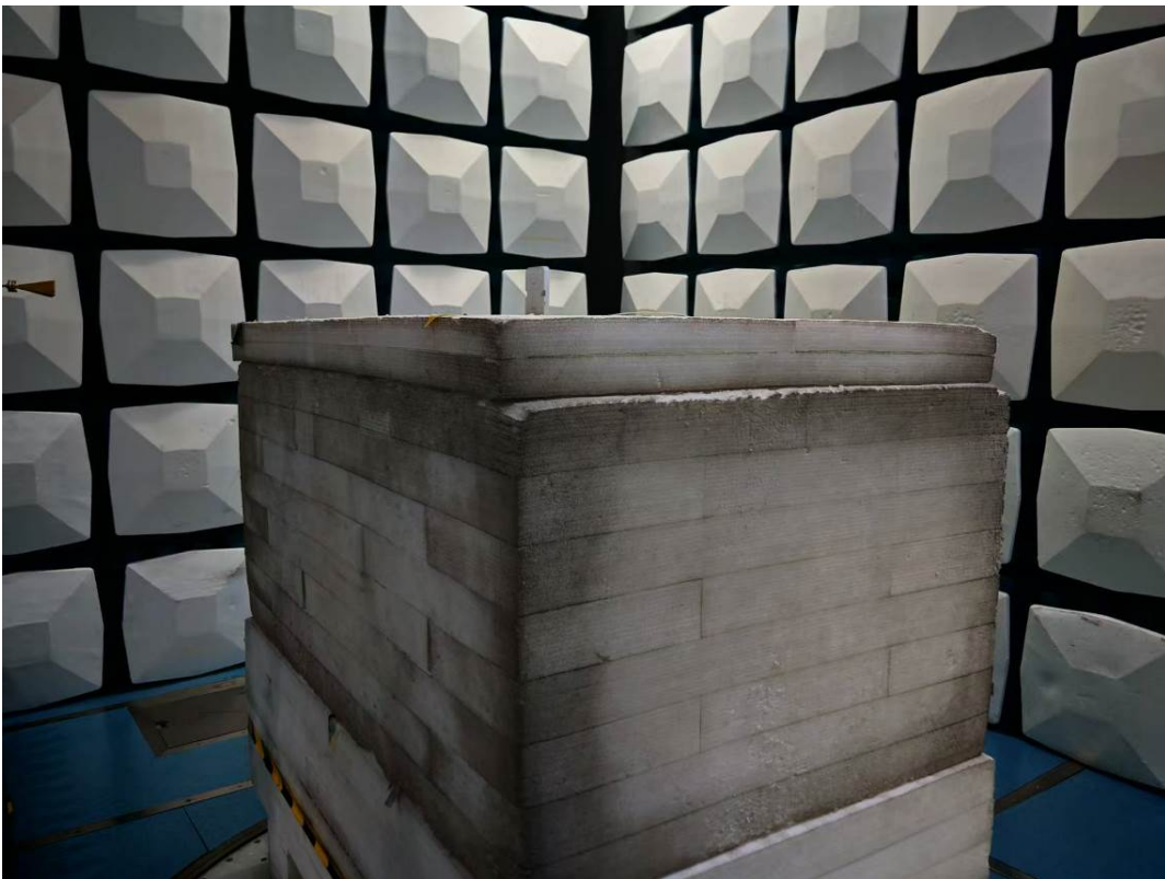
Radiated Emission 60-90GHz View
