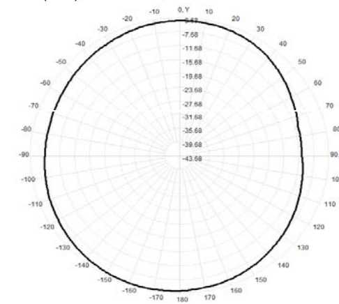
Total(H-XY), Max= -4.31dBi, CirD=6.75
