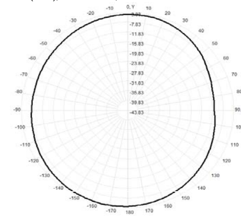
Total(H-XY), Max= -4.40dBi, CirD=6.95
