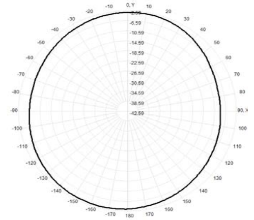
Total(H-XY), Max= -3.20dBi, CirD=5.45
