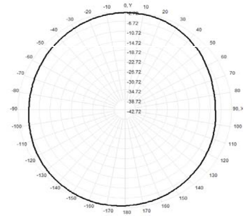
Total(H-XY), Max= -3.26dBi, CirD=5.75
