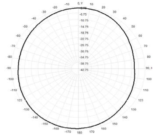
Total(H-XY), Max= -3.41dBi, CirD=5.96
