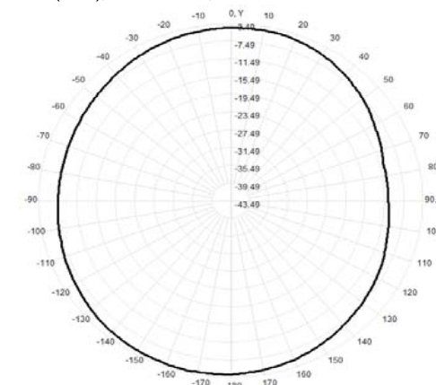
Total(H-XY), Max= -4.23dBi, CirD=6.60
