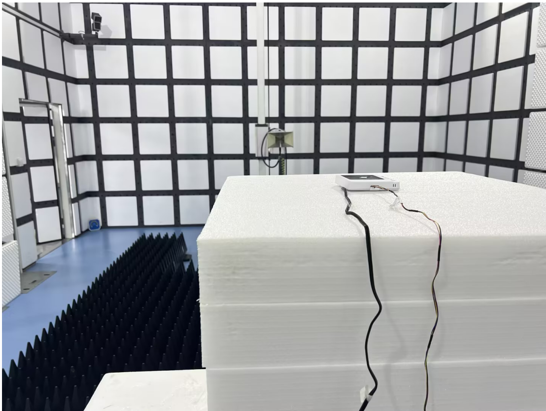
Radiated Emission - Front View (1 GHz-10 GHz)
