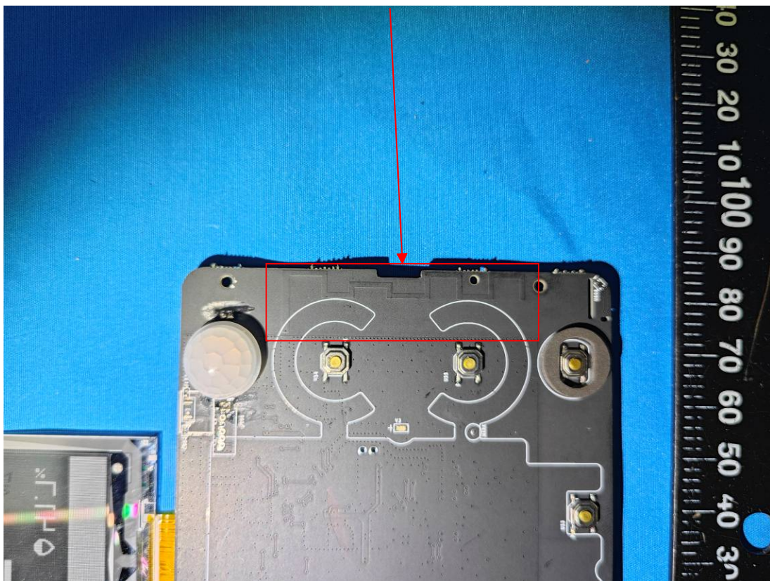
Lora&Bluetooth Antenna
