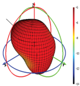
Freq=860MHz
