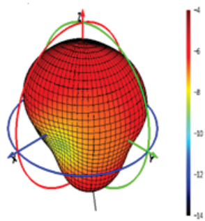
Freq=910MHz
