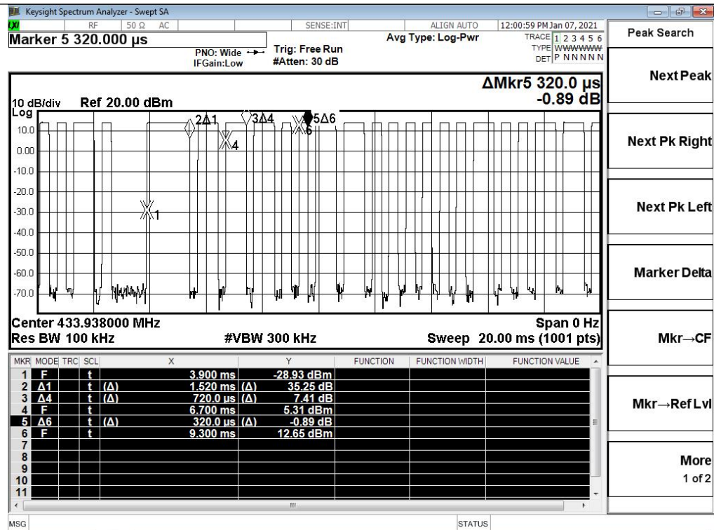
Fig.3 Pluse type 1 width=0.32ms Pluse type 2 width=0.72ms Pluse type 3width=1.52ms
