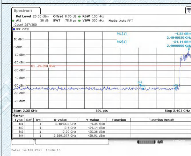
3DH5(2402)-Hopping on
