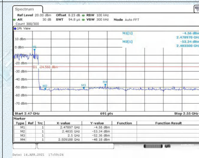
3DH5(2480)-Hopping on
