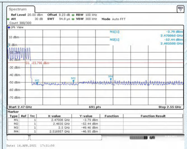
2DH5(2480)-Hopping on
