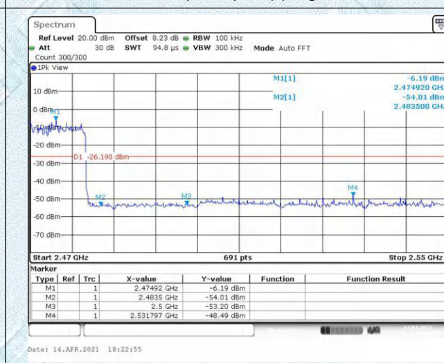
3DH5(2480)-Hopping on
