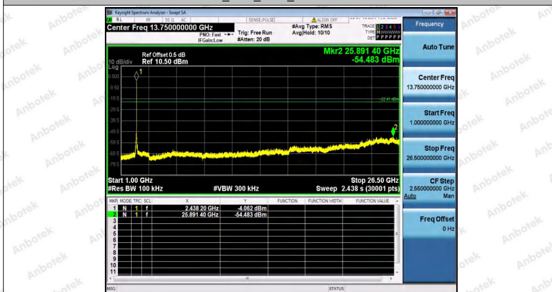
11G_Ant1_2437_1000~26500
