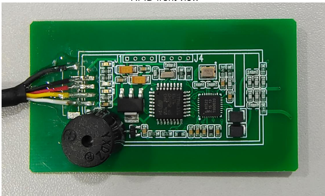
RFID front view
