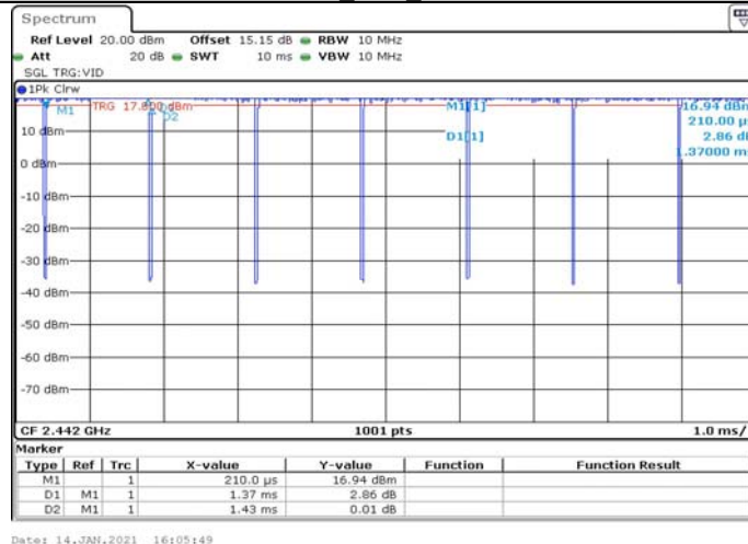
11N20SISO_Ant1_2442
