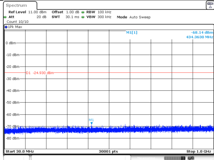
RF4CE_Ant1_2402 MHz_30~1000 MHz
