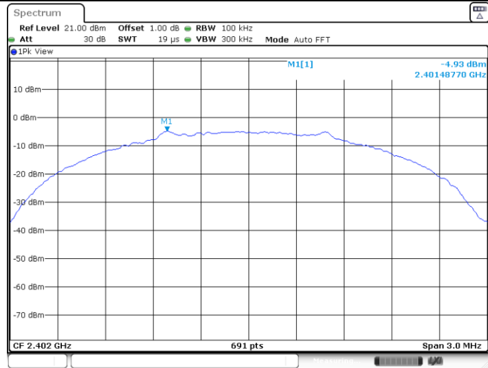
RF4CE_Ant1_2402 MHz_0~Reference
