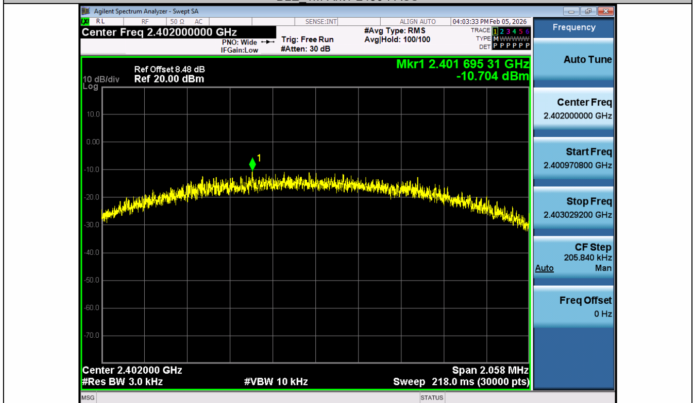
BLE_2M-Ant1-2402-PASS
