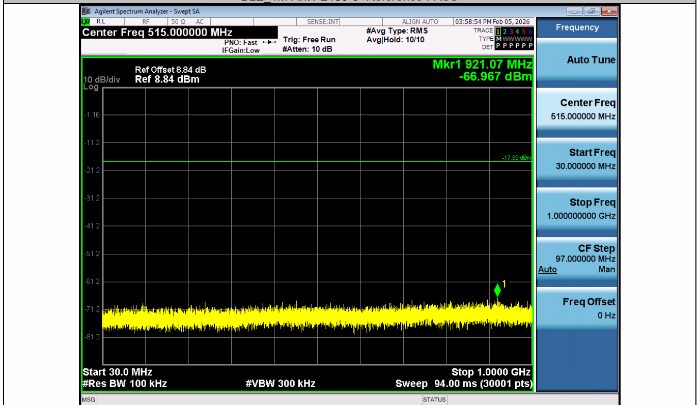
BLE_1M-Ant1-2480-30~1000-PASS
