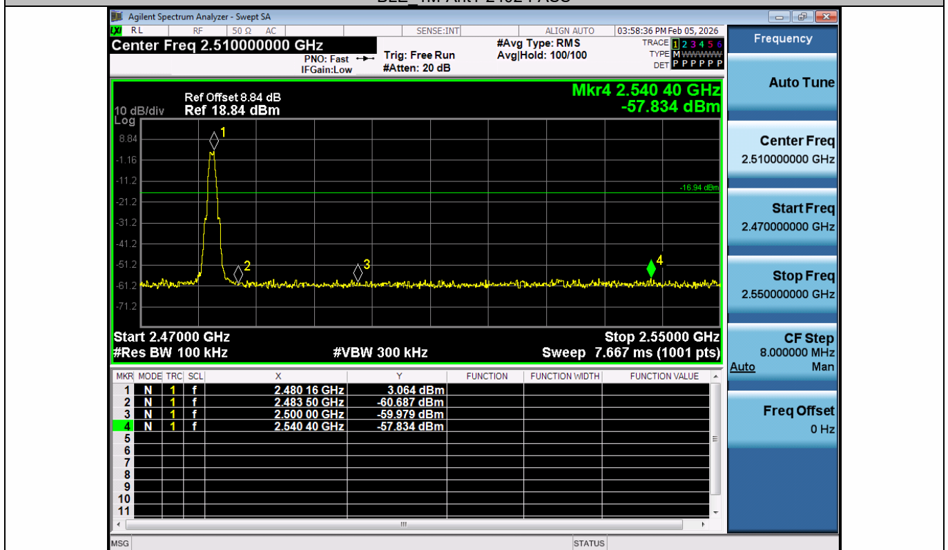
BLE_1M-Ant1-2480-PASS
