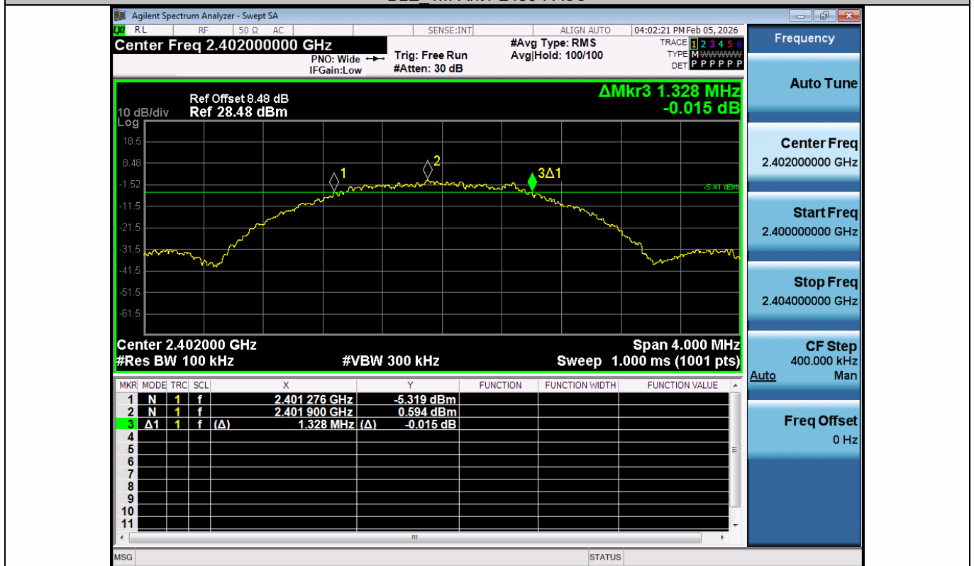
BLE_2M-Ant1-2402-PASS
