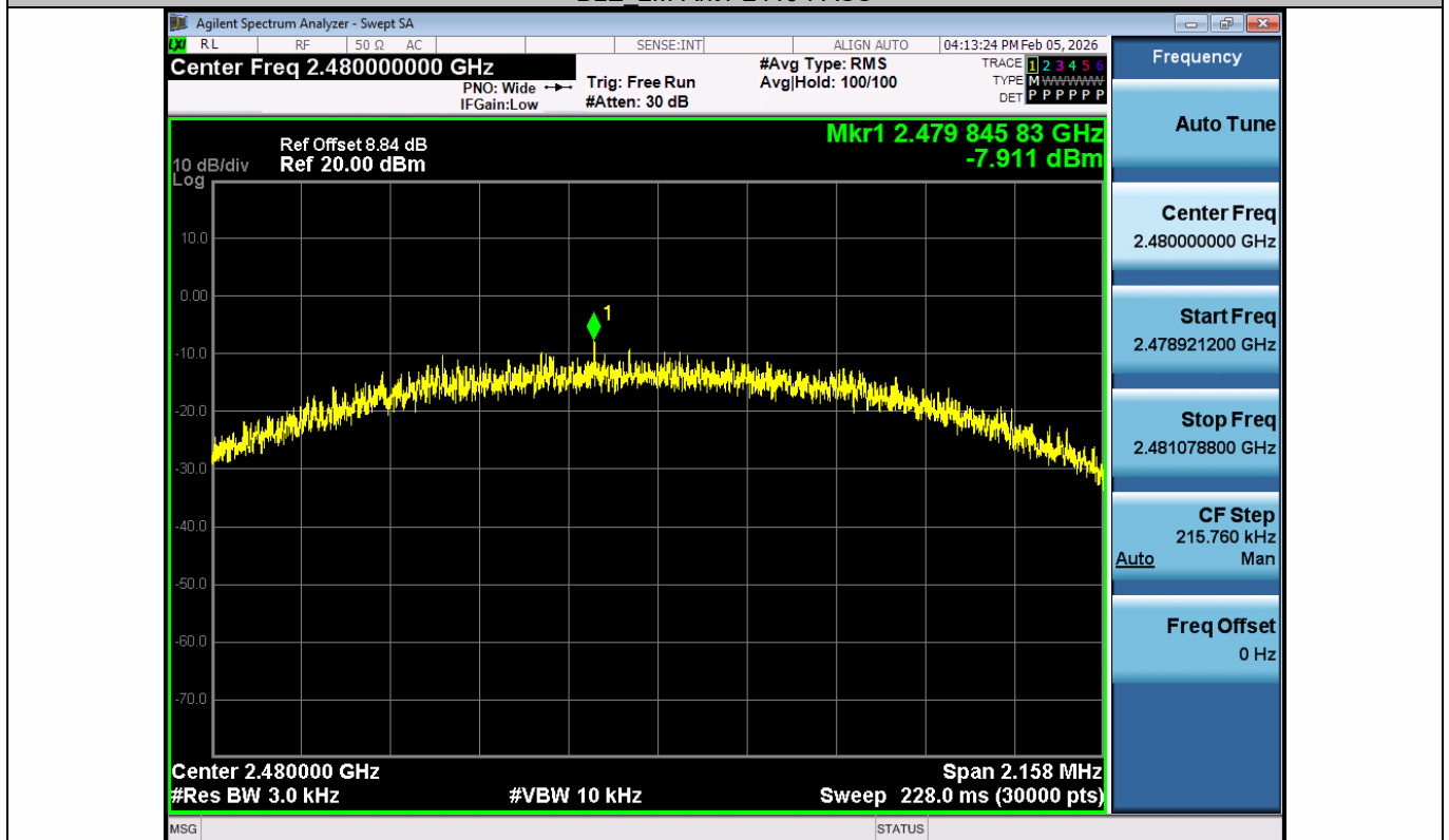
BLE_2M-Ant1-2480-PASS
