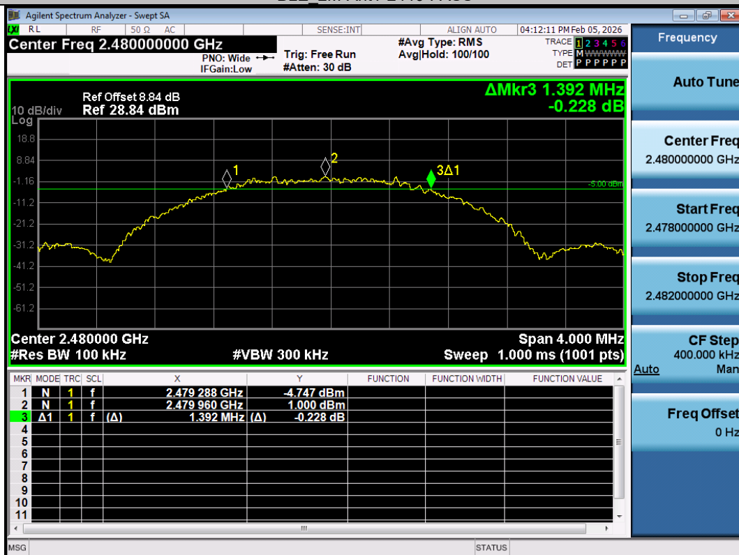
BLE_2M-Ant1-2480-PASS
