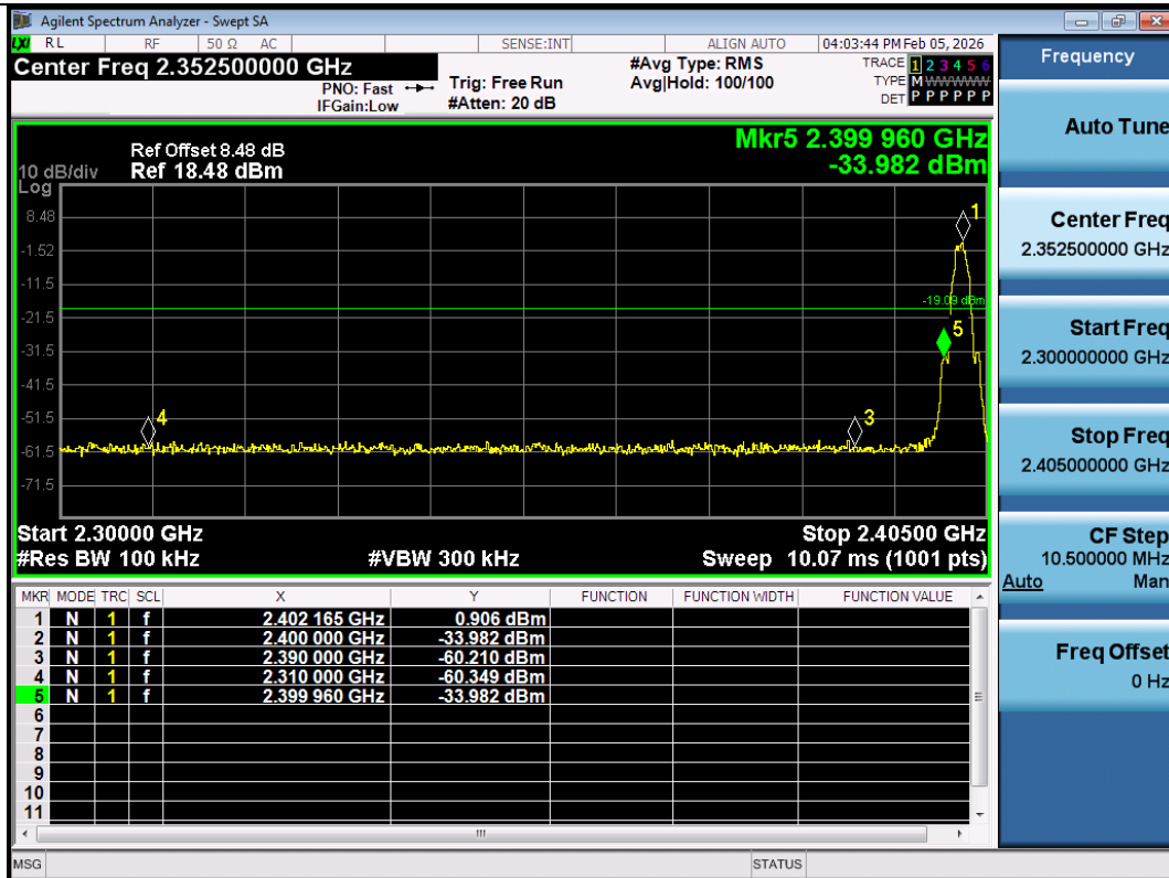
BLE_2M-Ant1-2402-PASS
