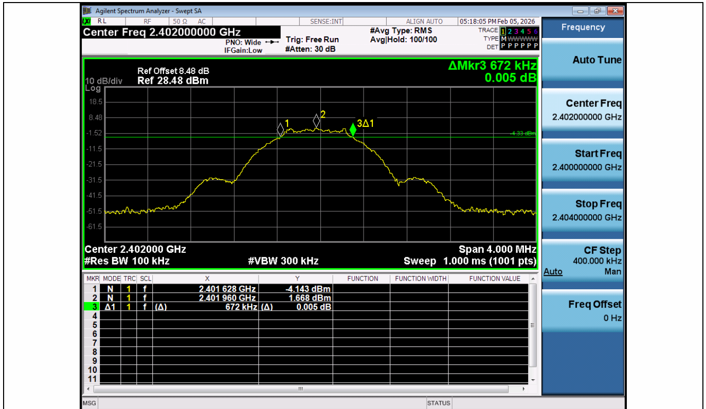
BLE_1M-Ant1-2402-PASS
