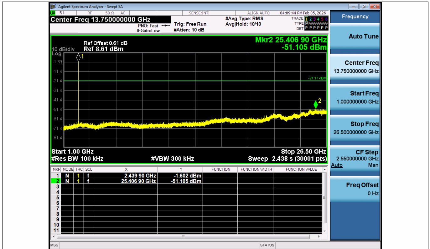
BLE_2M-Ant1-2440-1000~26500-PASS
