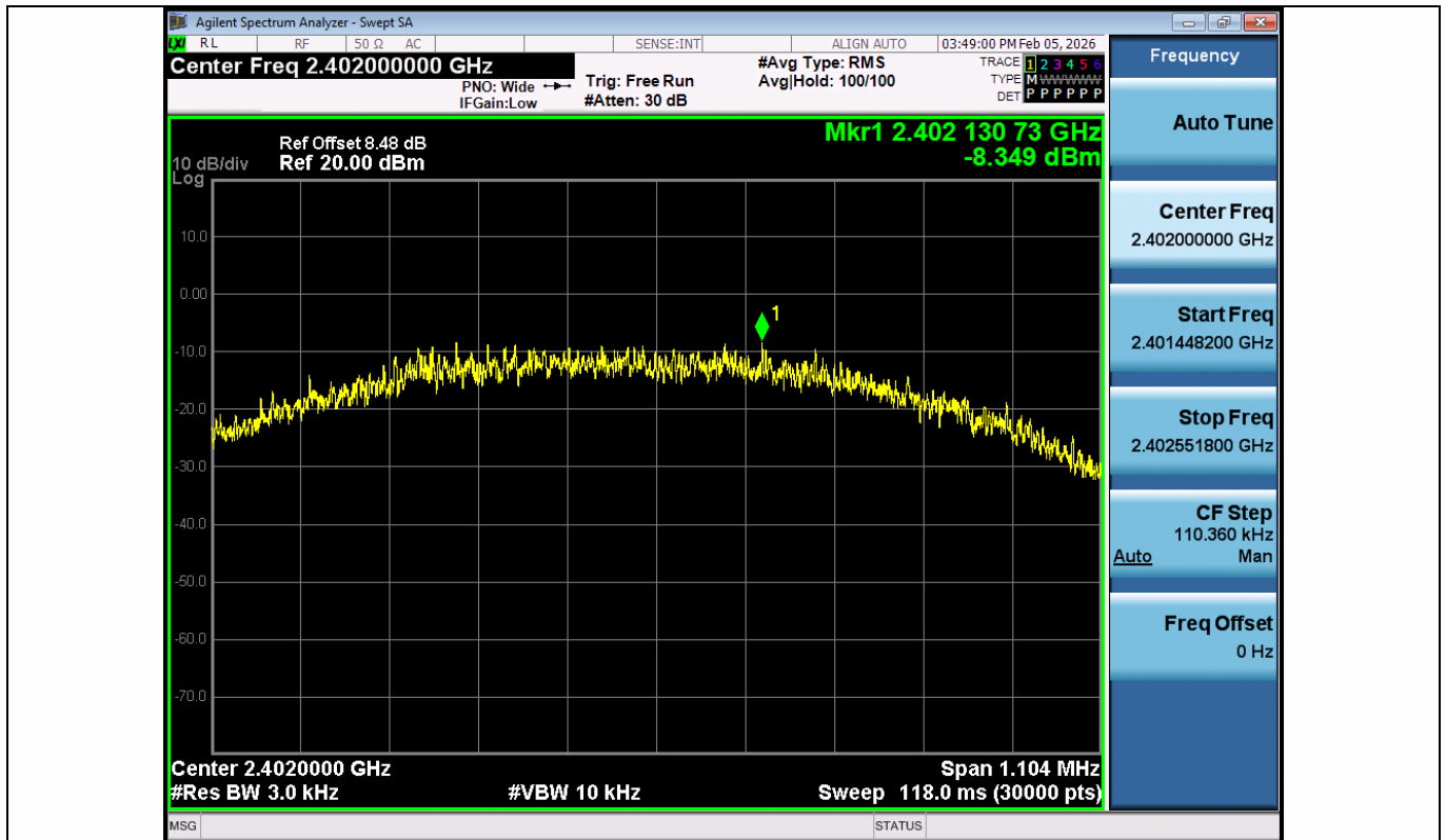
BLE_1M-Ant1-2402-PASS
