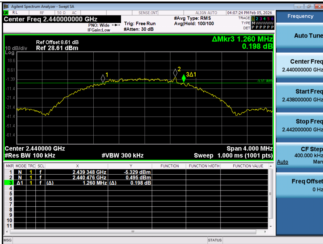
BLE_2M-Ant1-2440-PASS
