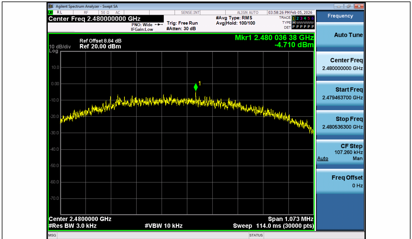
BLE_1M-Ant1-2480-PASS
