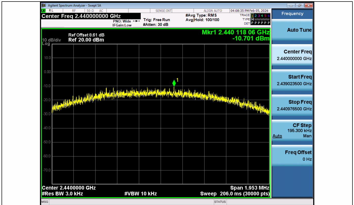
BLE_2M-Ant1-2440-PASS
