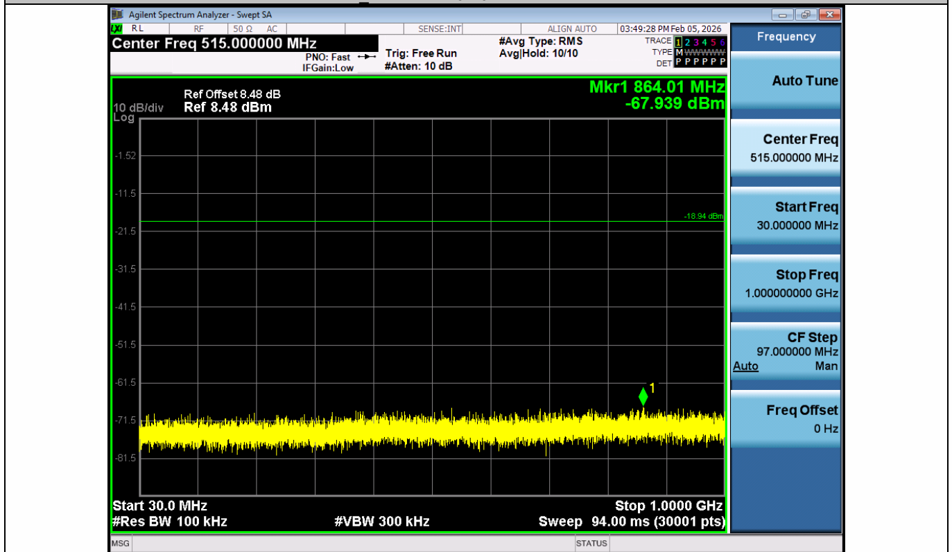
BLE_1M-Ant1-2402-30~1000-PASS
