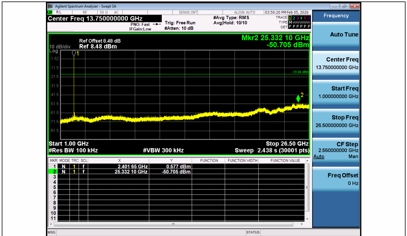
BLE_1M-Ant1-2402-1000~26500-PASS
