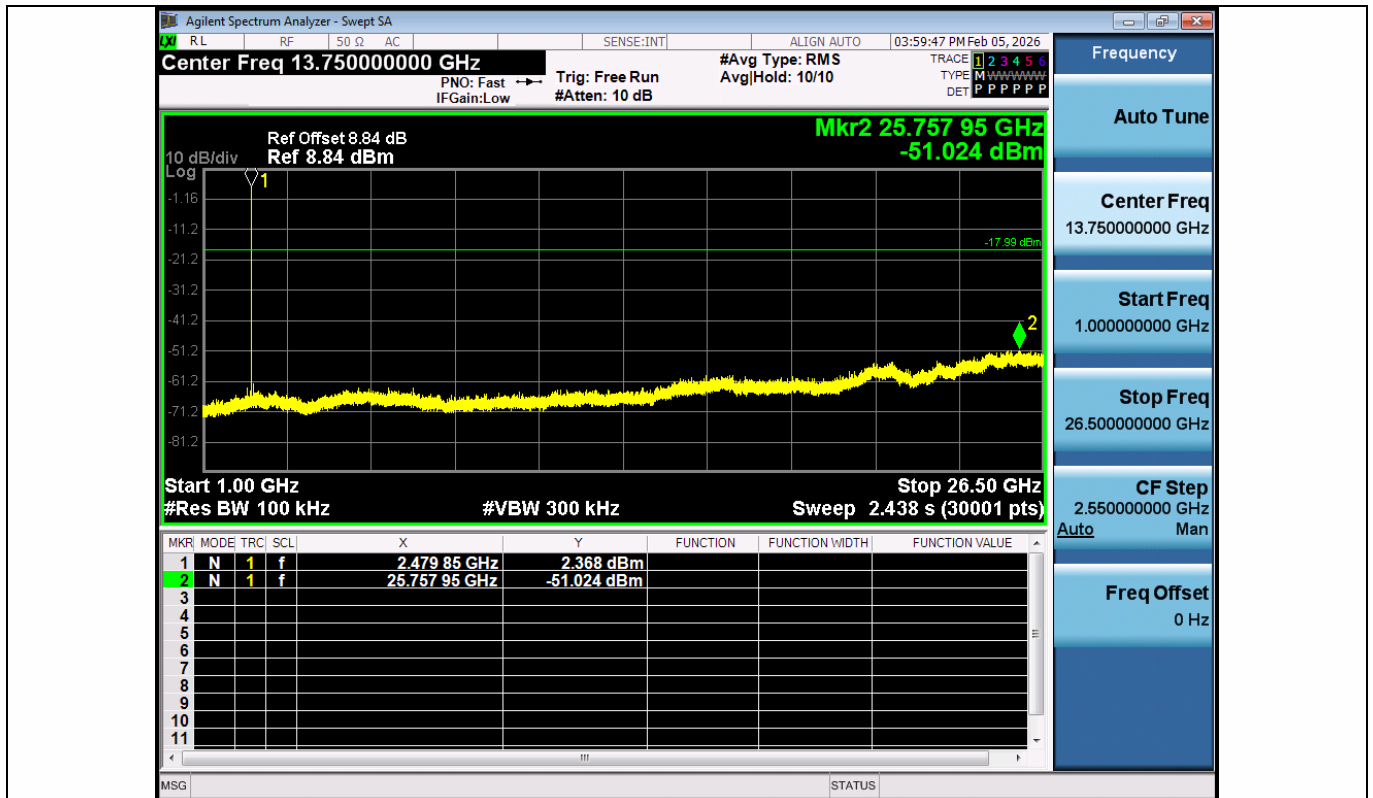
BLE_1M-Ant1-2480-1000~26500-PASS
