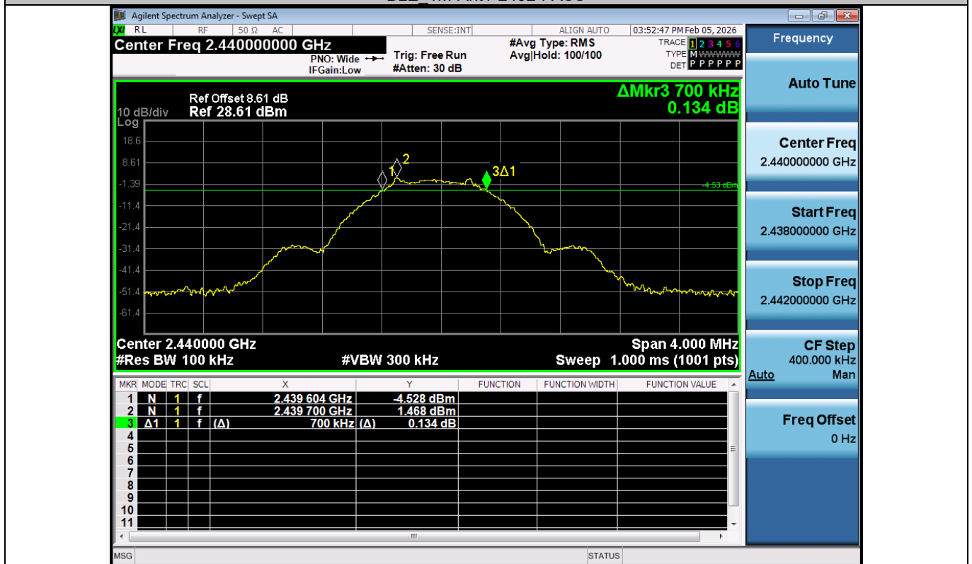
BLE_1M-Ant1-2440-PASS
