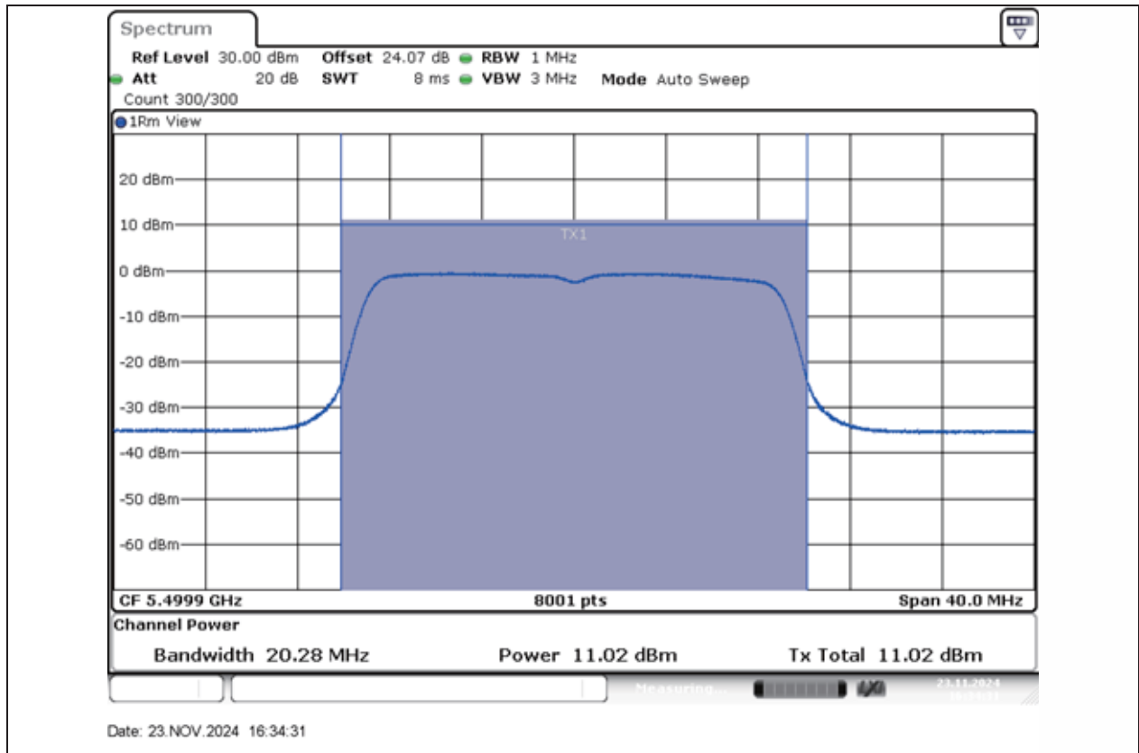
11AC20MIMO-Ant1-5500-PASS
