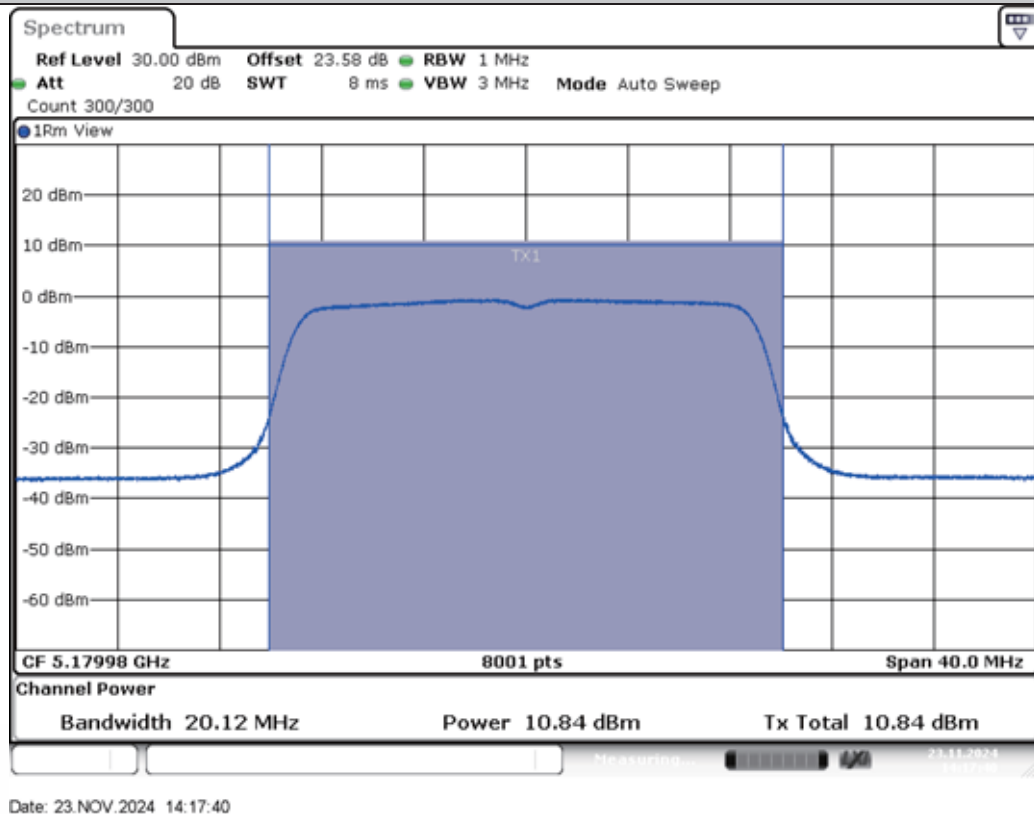
11N20MIMO-Ant2-5180-PASS
