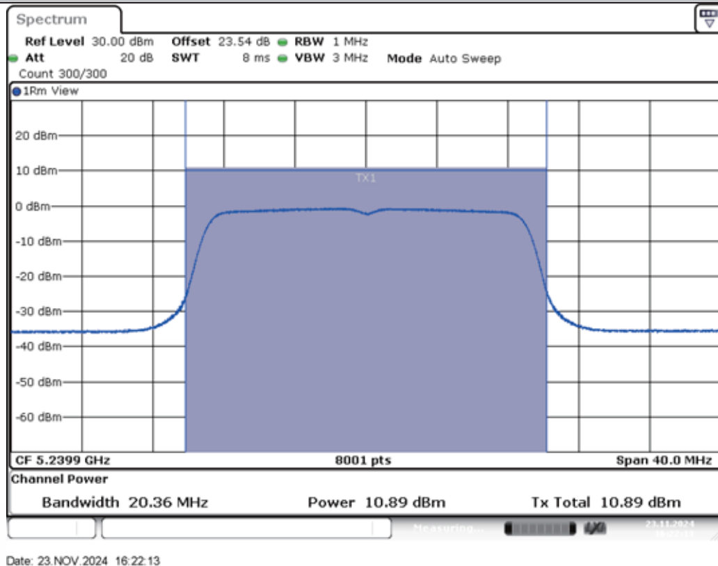
11AC20MIMO-Ant2-5240-PASS
