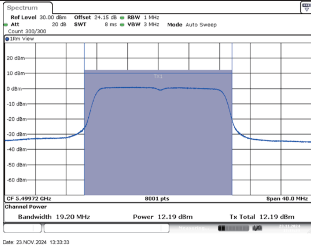
11A-Ant2-5500-PASS
