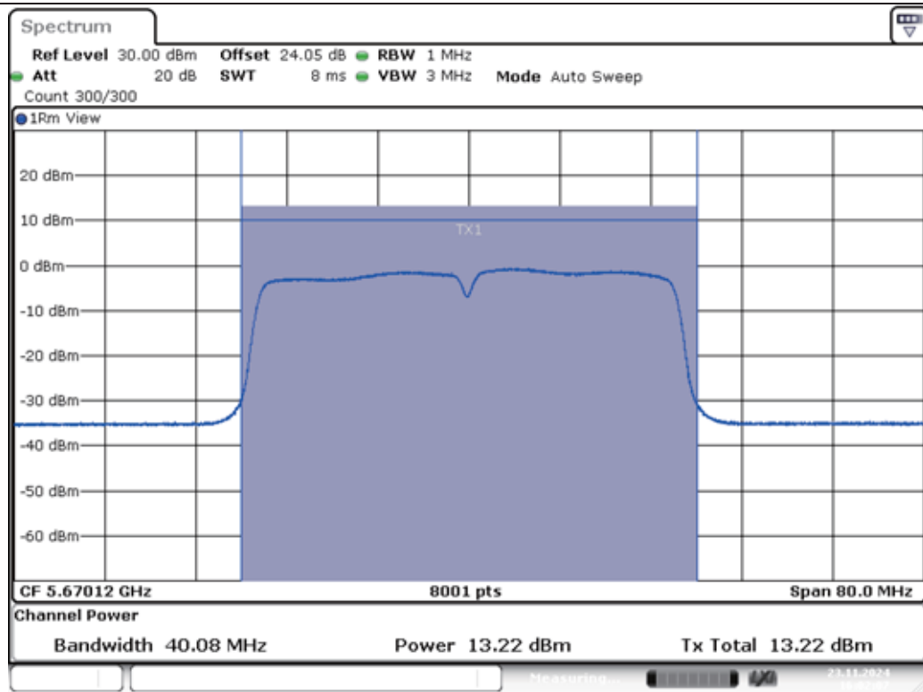
11N40MIMO-Ant1-5670-PASS
