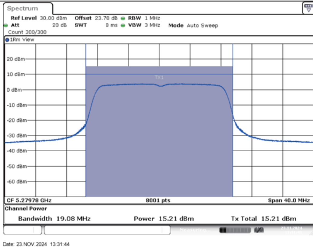
11A-Ant2-5280-PASS
