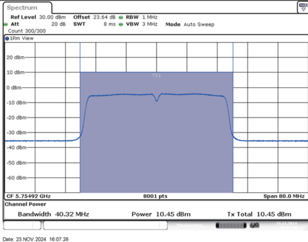
11N40MIMO-Ant2-5755-PASS
