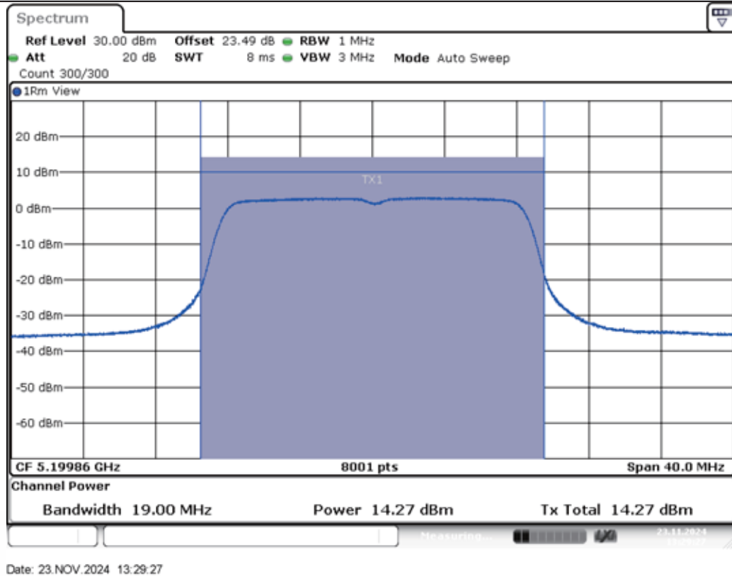
11A-Ant2-5200-PASS
