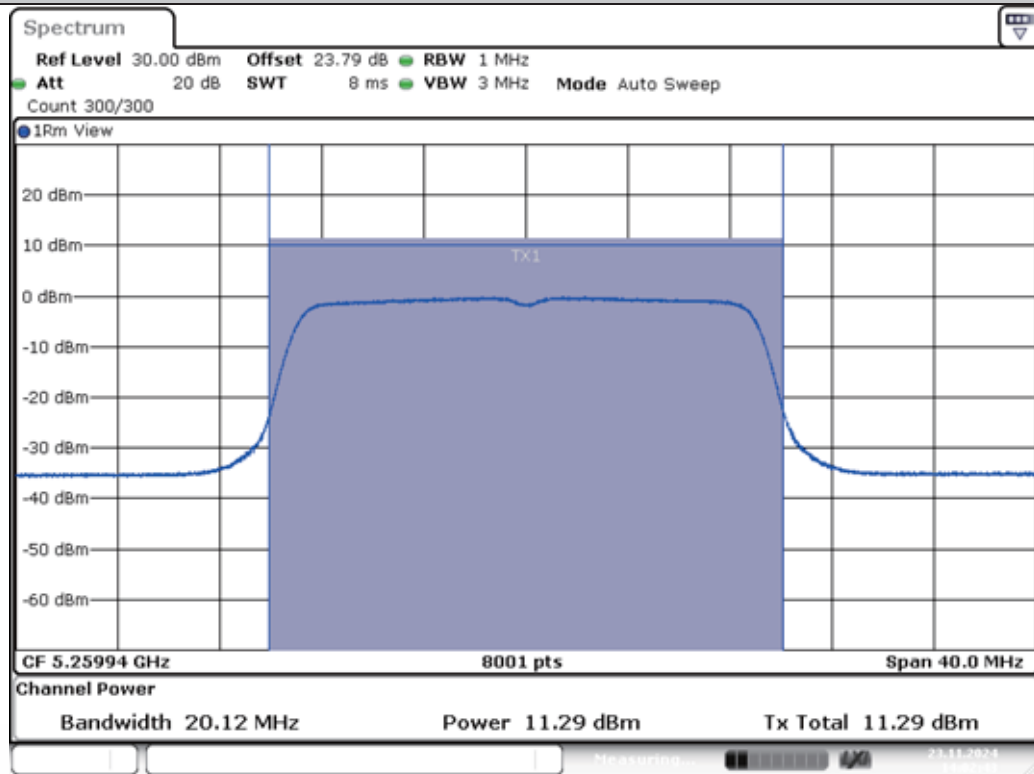
11N20MIMO-Ant1-5260-PASS
