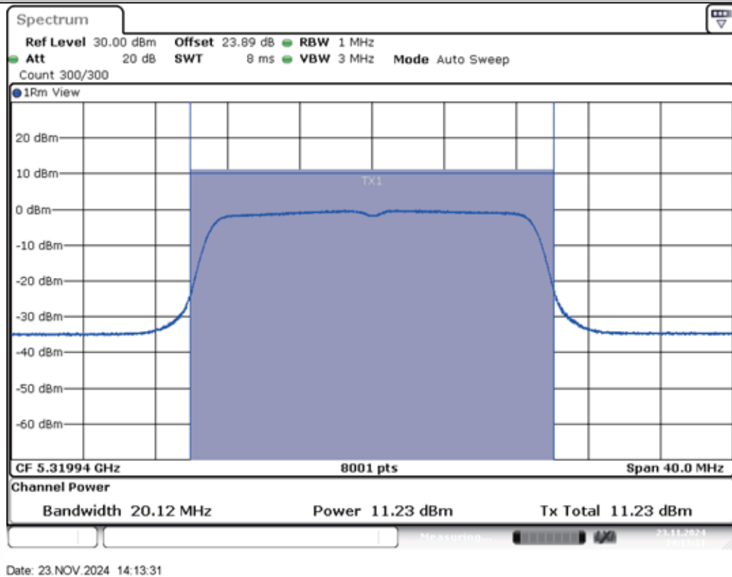
11N20MIMO-Ant2-5320-PASS
