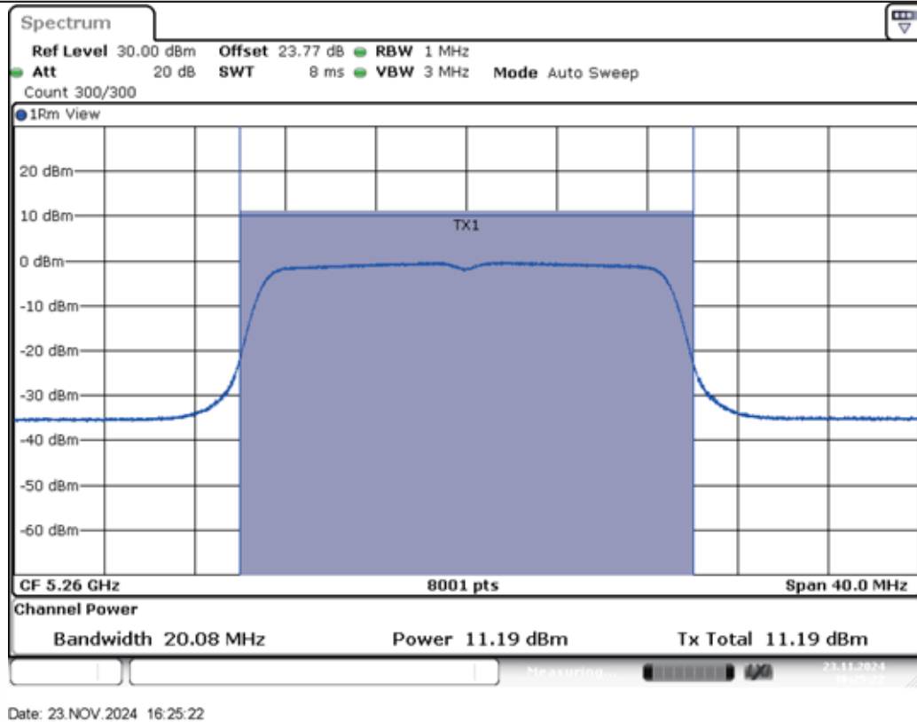
11AC20MIMO-Ant2-5260-PASS
