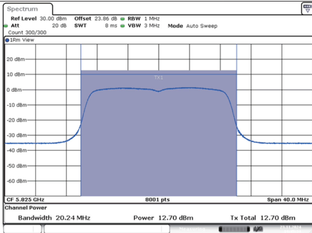
11N20MIMO-Ant1-5825-PASS
