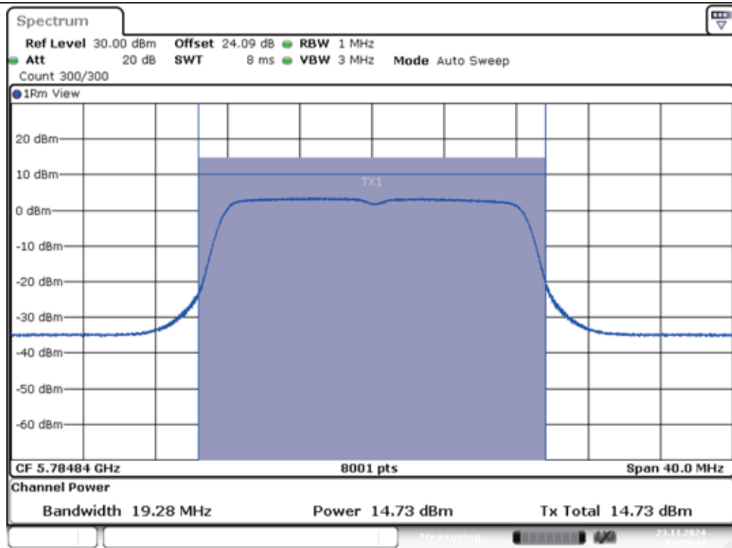
11A-Ant1-5785-PASS
