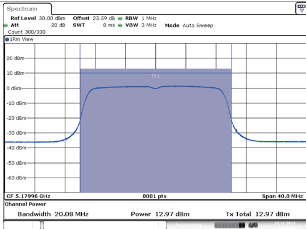
11N20MIMO-Ant1-5180-PASS
