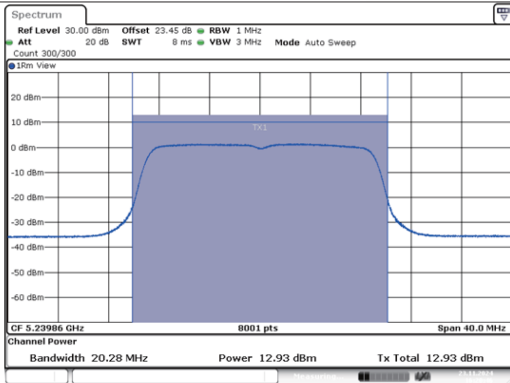
11AC20MIMO-Ant1-5240-PASS
