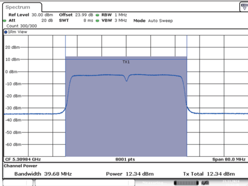
11N40MIMO-Ant1-5310-PASS
