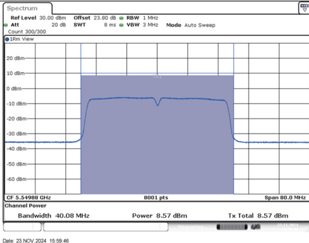
11N40MIMO-Ant2-5550-PASS
