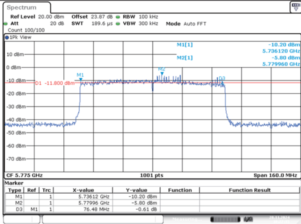
11AX80MIMO-Ant1-5775-PASS
