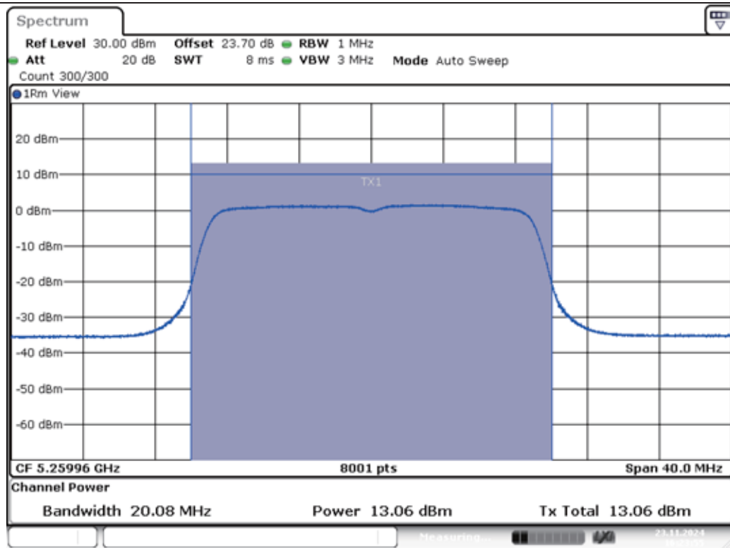
11AC20MIMO-Ant1-5260-PASS
