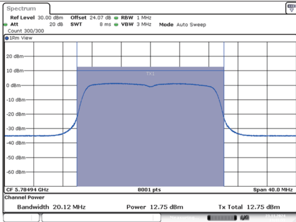
11N20MIMO-Ant1-5785-PASS
