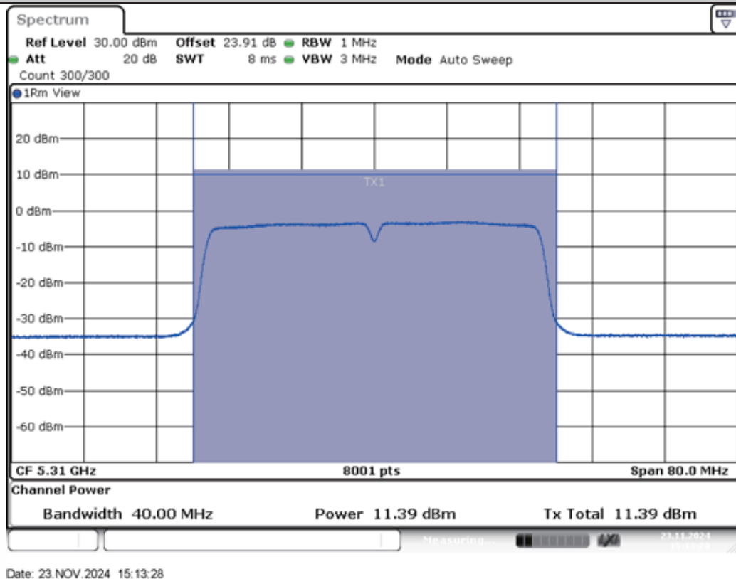
11N40MIMO-Ant2-5310-PASS
