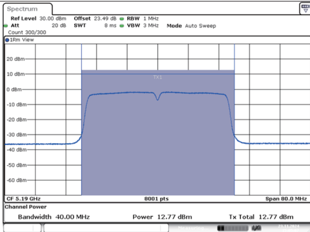
11N40MIMO-Ant1-5190-PASS
