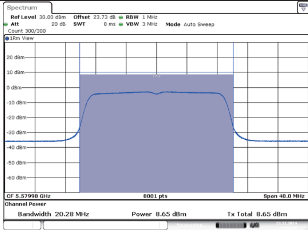
11N20MIMO-Ant1-5580-PASS
