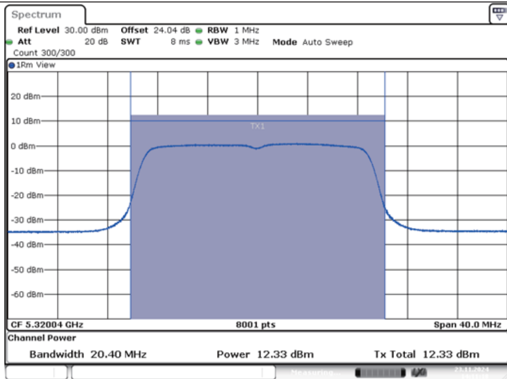
11N20MIMO-Ant1-5320-PASS
