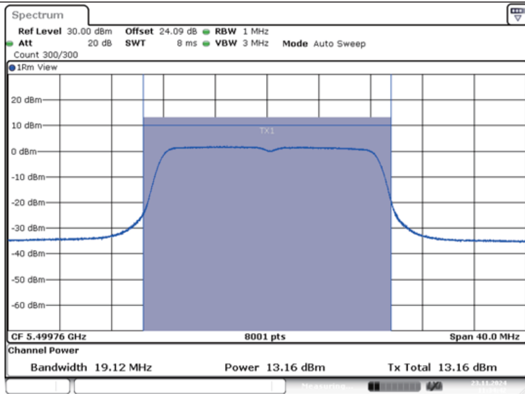
11A-Ant1-5500-PASS
