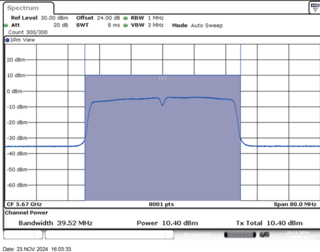
11N40MIMO-Ant2-5670-PASS
