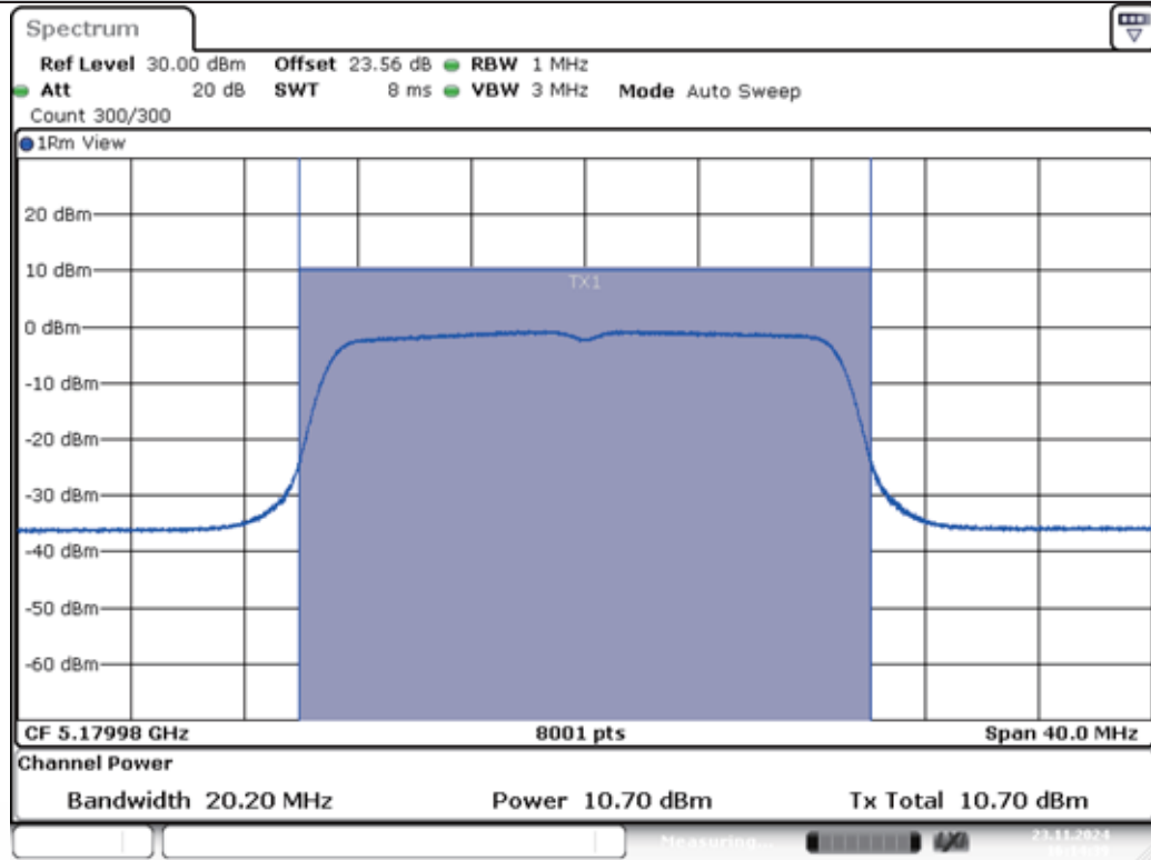
11AC20MIMO-Ant1-5180-PASS
