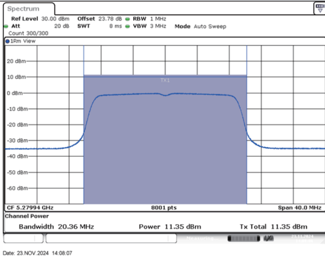
11N20MIMO-Ant2-5280-PASS
