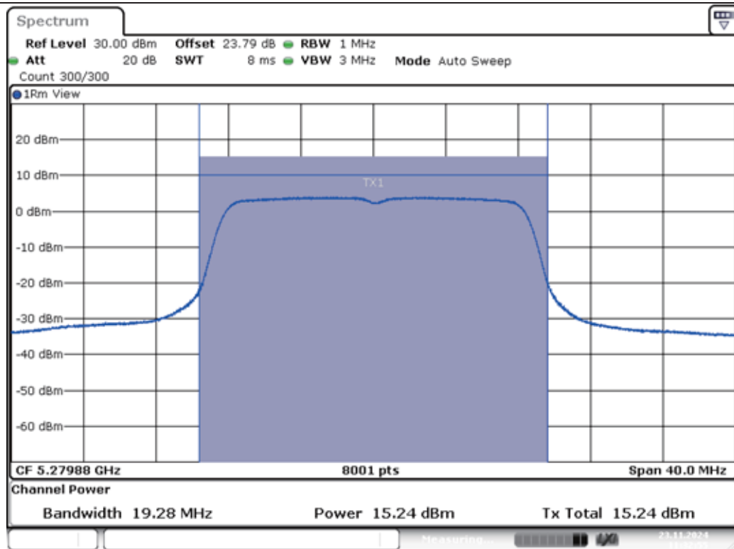
11A-Ant1-5280-PASS
