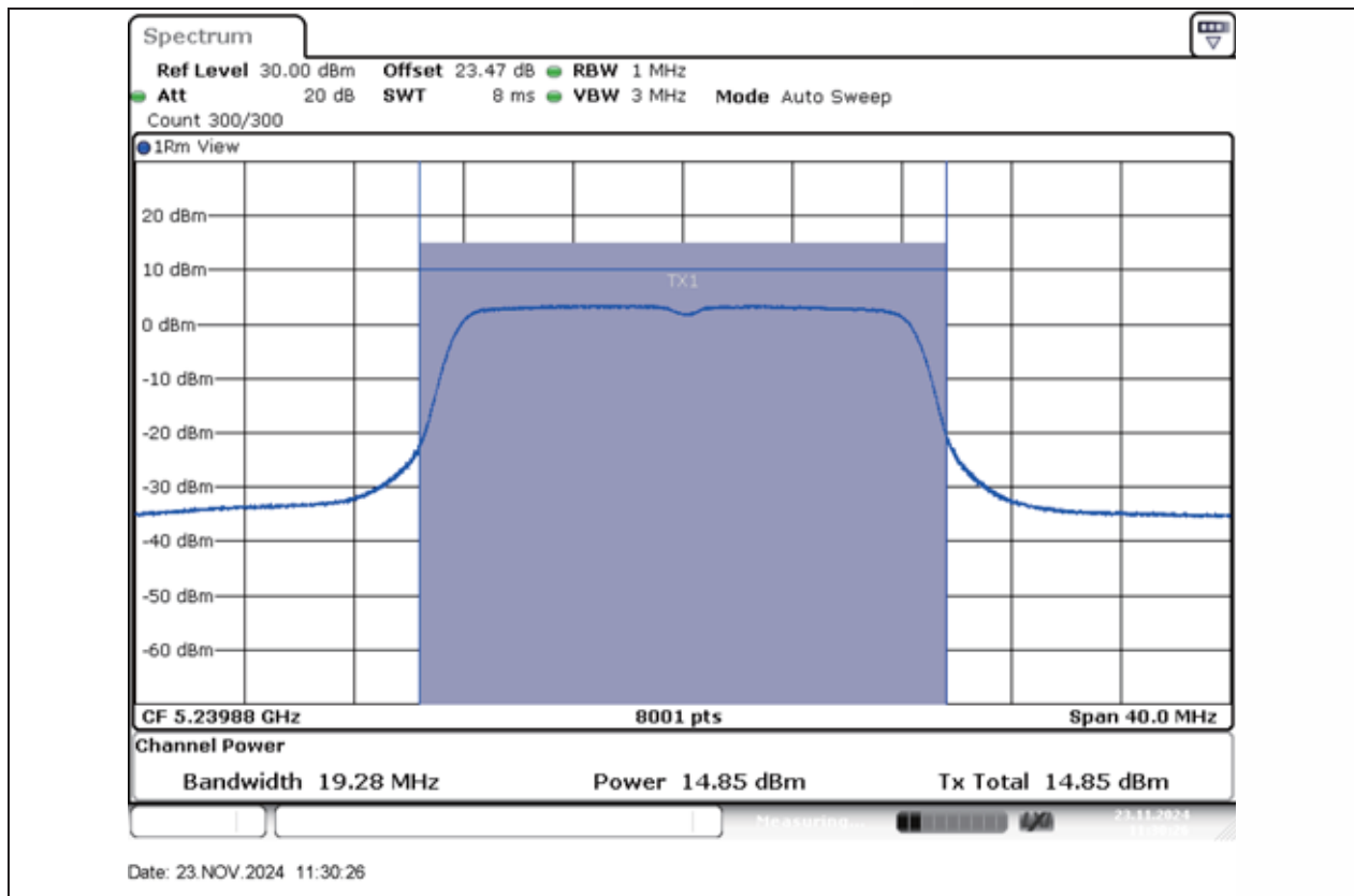
11A-Ant1-5240-PASS
