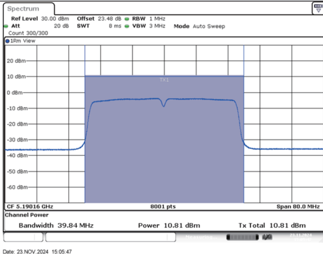
11N40MIMO-Ant2-5190-PASS
