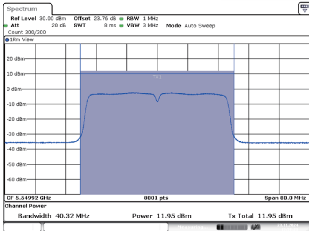
11N40MIMO-Ant1-5550-PASS
