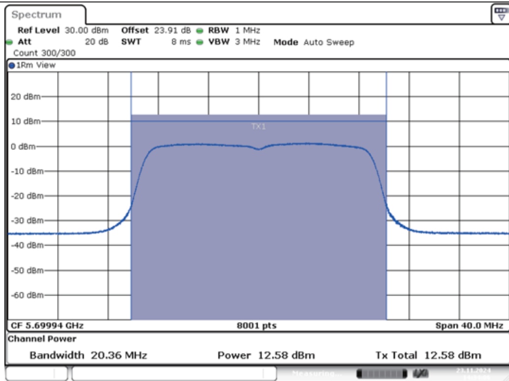
11N20MIMO-Ant1-5700-PASS
