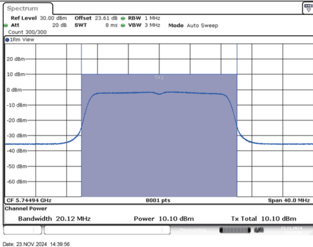
11N20MIMO-Ant2-5745-PASS
