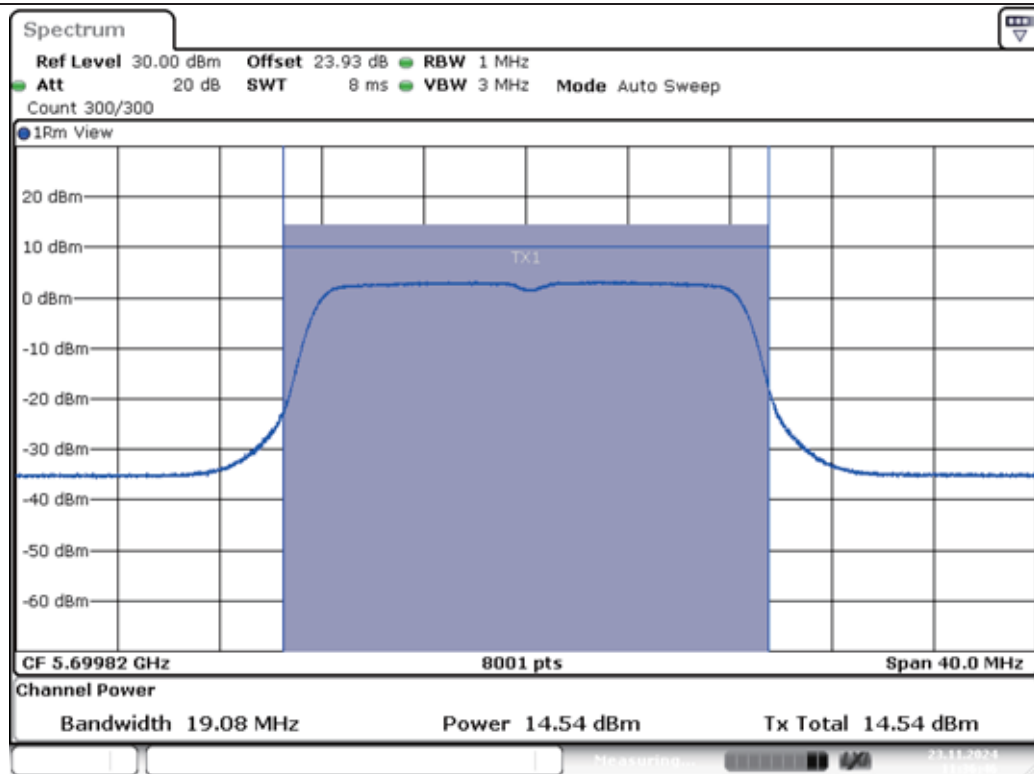
11A-Ant1-5700-PASS
