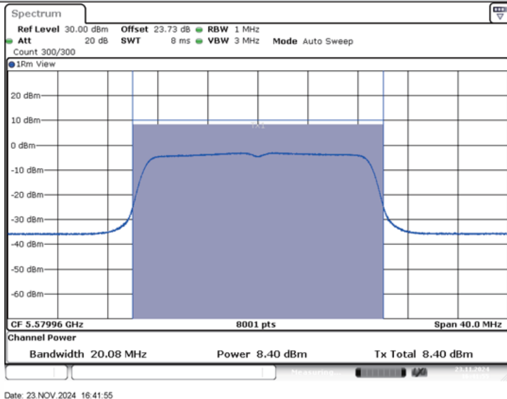
11AC20MIMO-Ant2-5580-PASS
