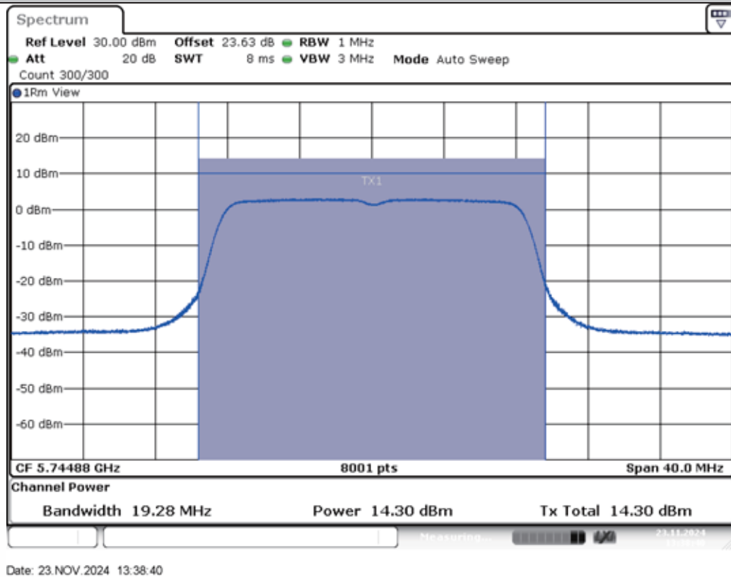
11A-Ant2-5745-PASS
