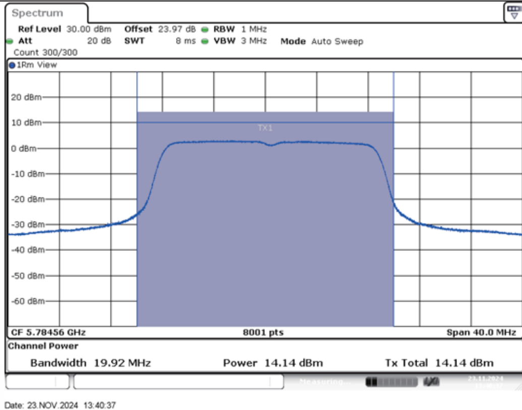
11A-Ant2-5785-PASS
