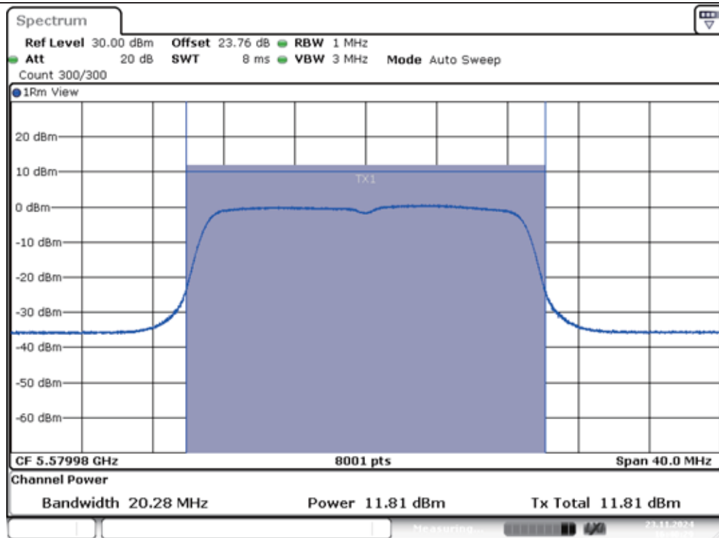
11AC20MIMO-Ant1-5580-PASS
