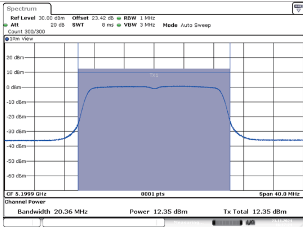
11AC20MIMO-Ant1-5200-PASS
