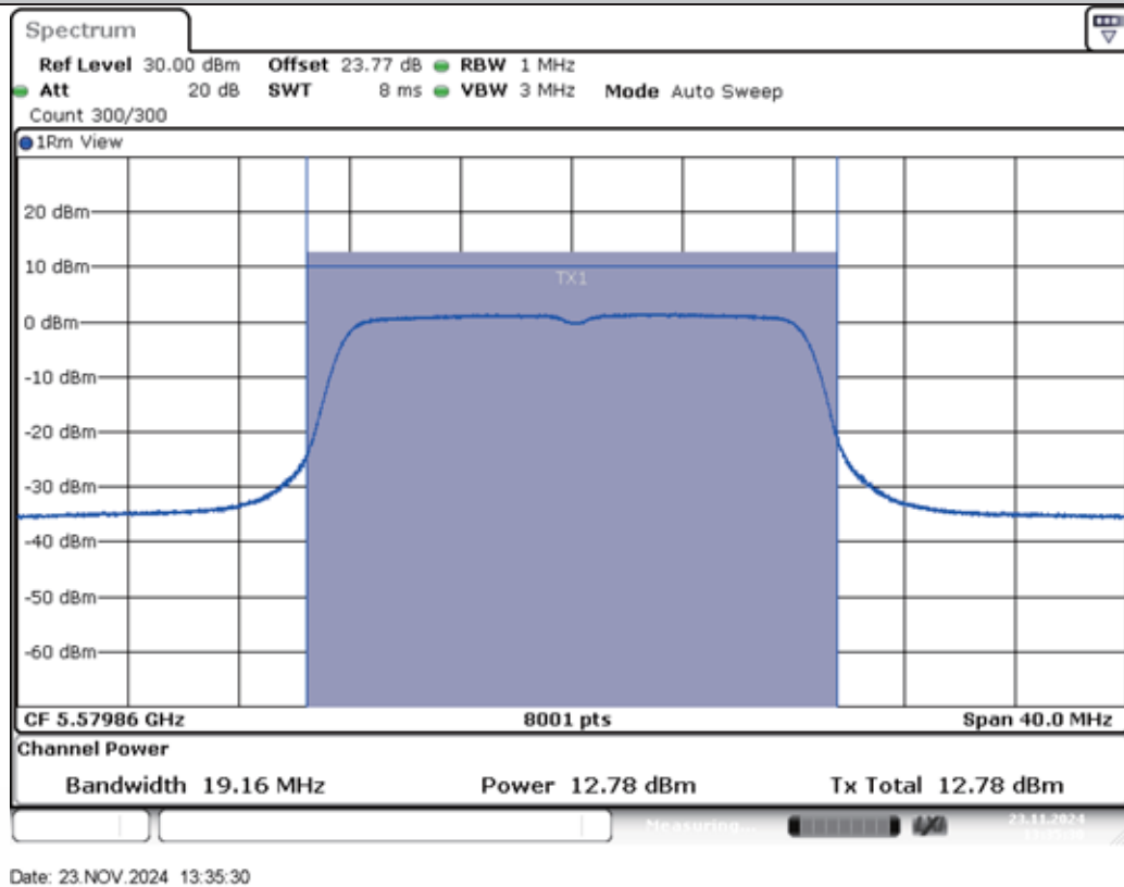
11A-Ant2-5580-PASS
