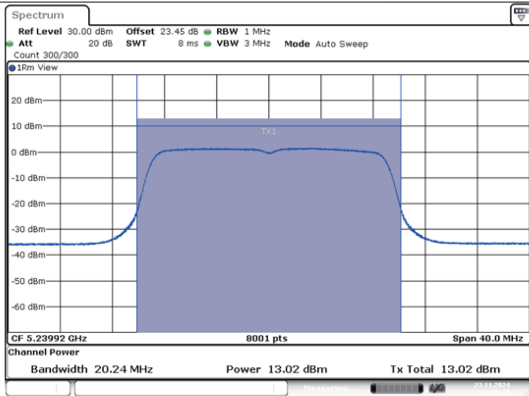
11N20MIMO-Ant1-5240-PASS
