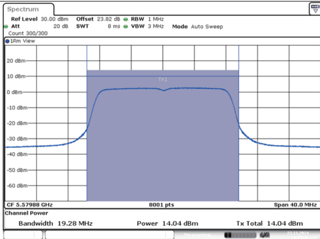
11A-Ant1-5580-PASS
