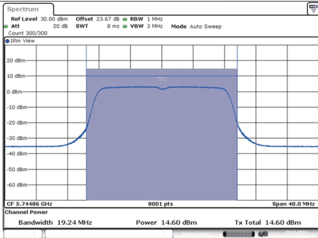
11A-Ant1-5745-PASS
