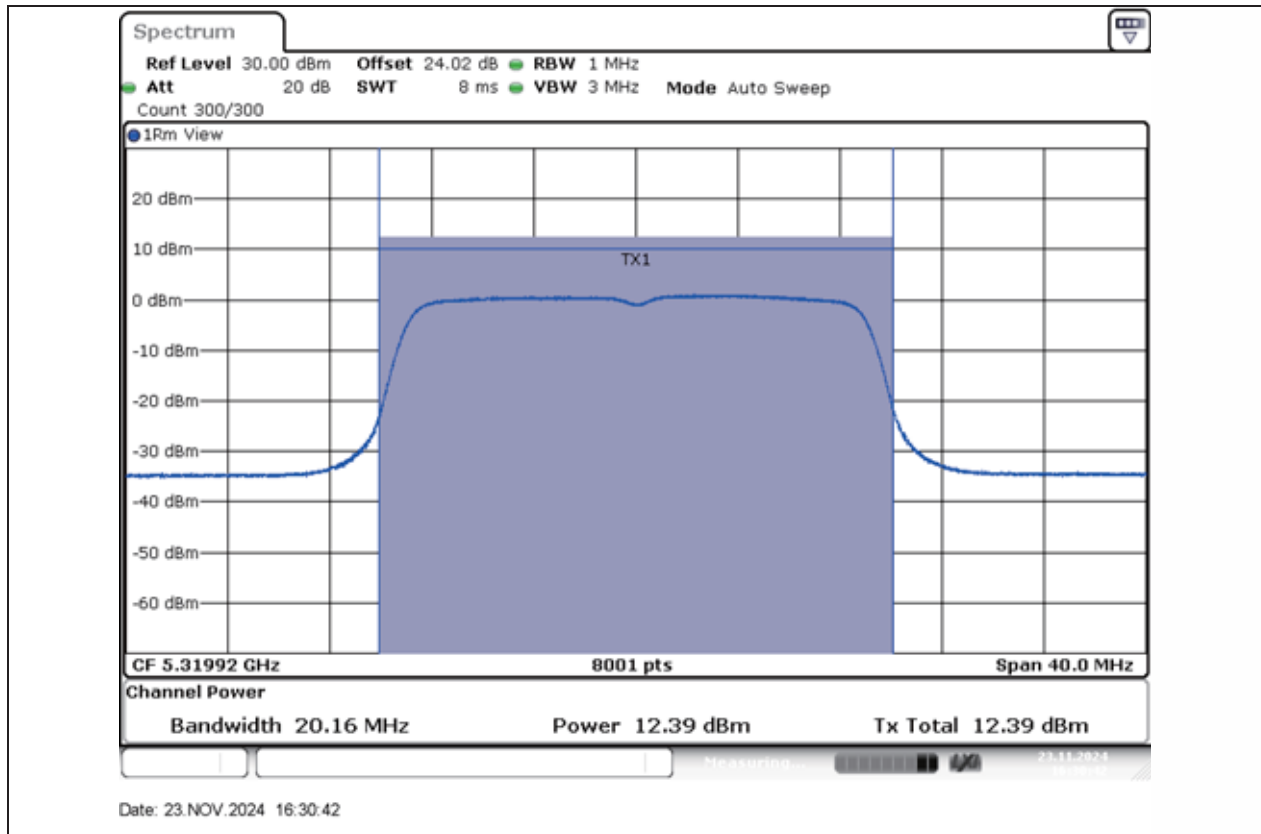
11AC20MIMO-Ant1-5320-PASS
