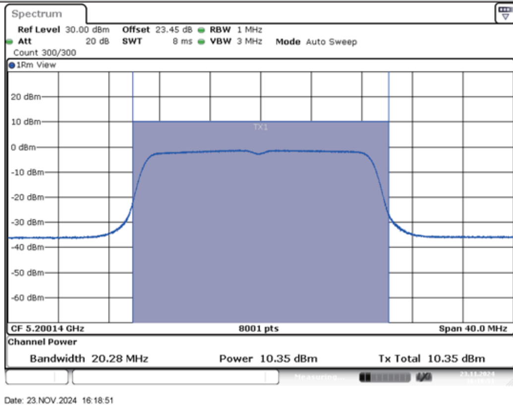
11AC20MIMO-Ant2-5200-PASS
