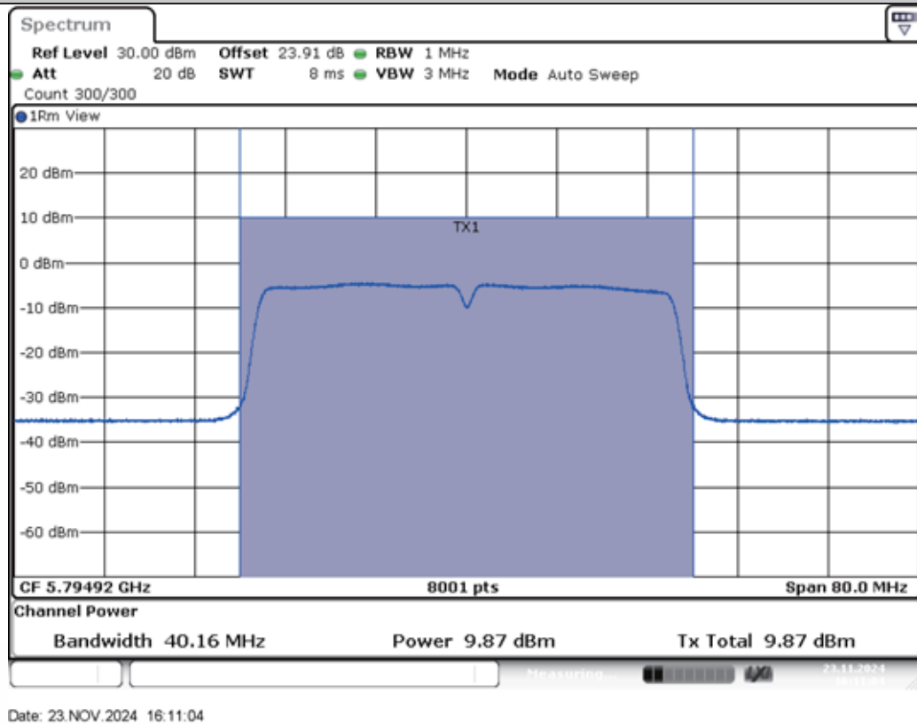
11N40MIMO-Ant2-5795-PASS
