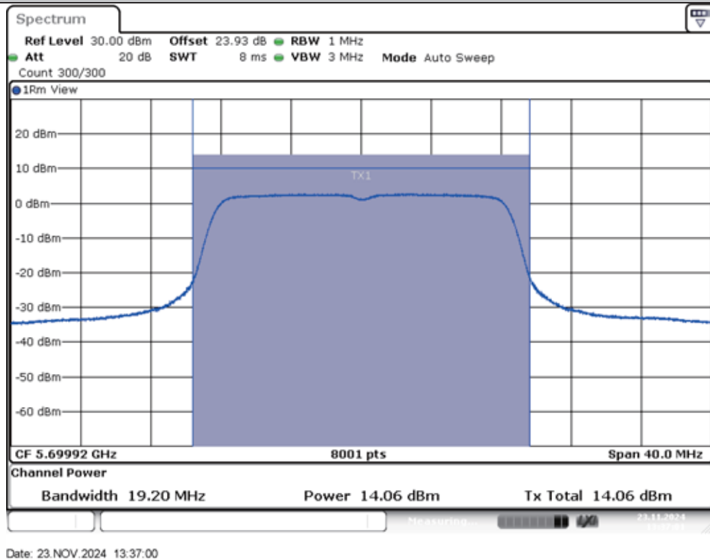
11A-Ant2-5700-PASS
