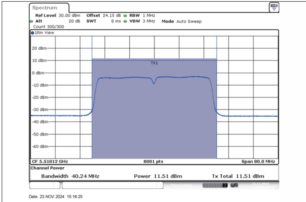
11N40MIMO-Ant1-5510-PASS
