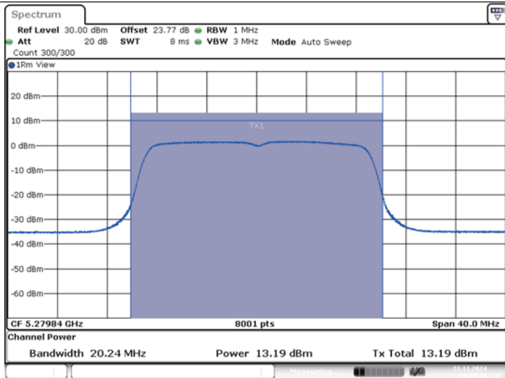
11N20MIMO-Ant1-5280-PASS
