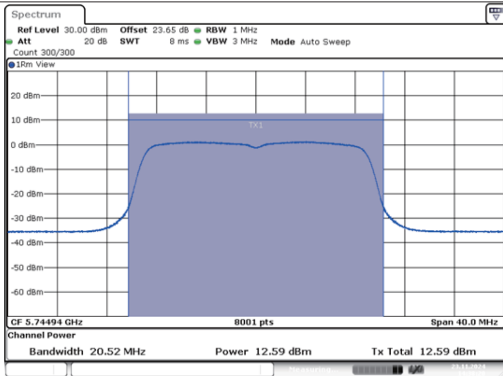
11N20MIMO-Ant1-5745-PASS
