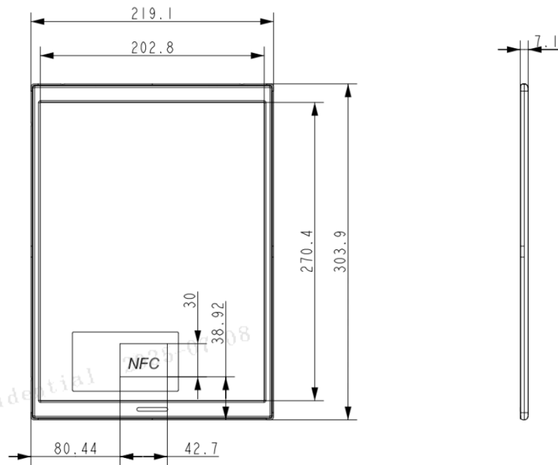
Figure 2-3 31.5" dimensions
