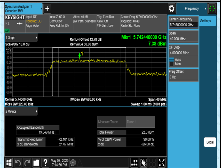
11AX20SISO-Ant1-5745
