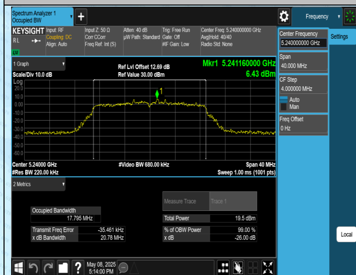
11AC20SISO-Ant1-5240
