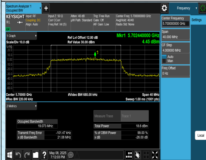
11AX20SISO-Ant1-5700
