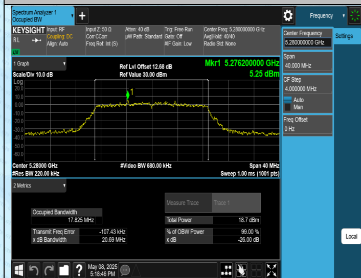
11AC20SISO-Ant1-5280
