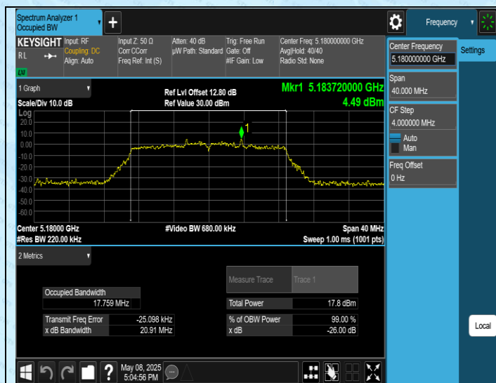
11AC20SISO-Ant1-5180
