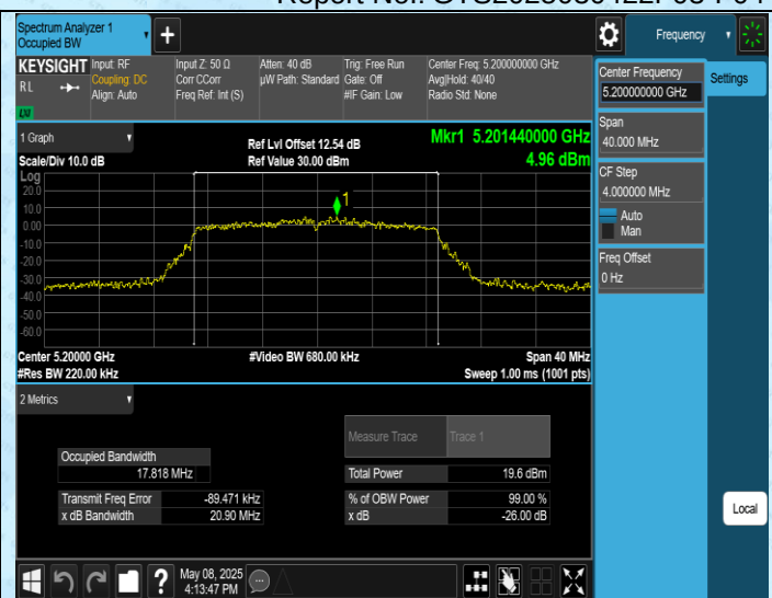
11N20SISO-Ant1-5200
