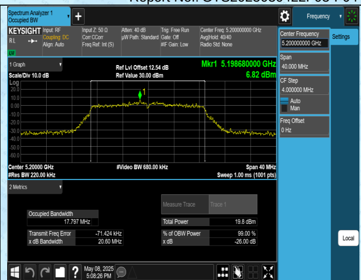
11AC20SISO-Ant1-5200
