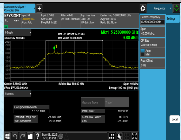
11AC20SISO-Ant1-5260
