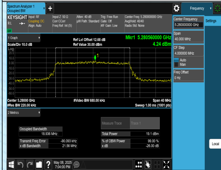
11AX20SISO-Ant1-5280
