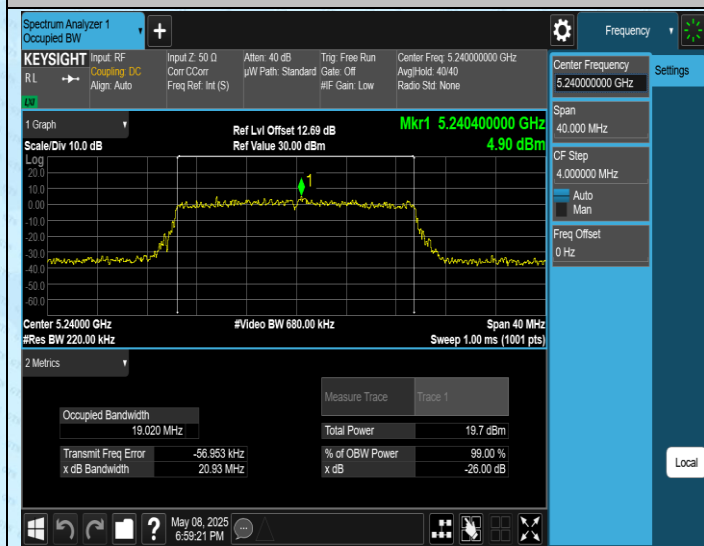
11AX20SISO-Ant1-5240
