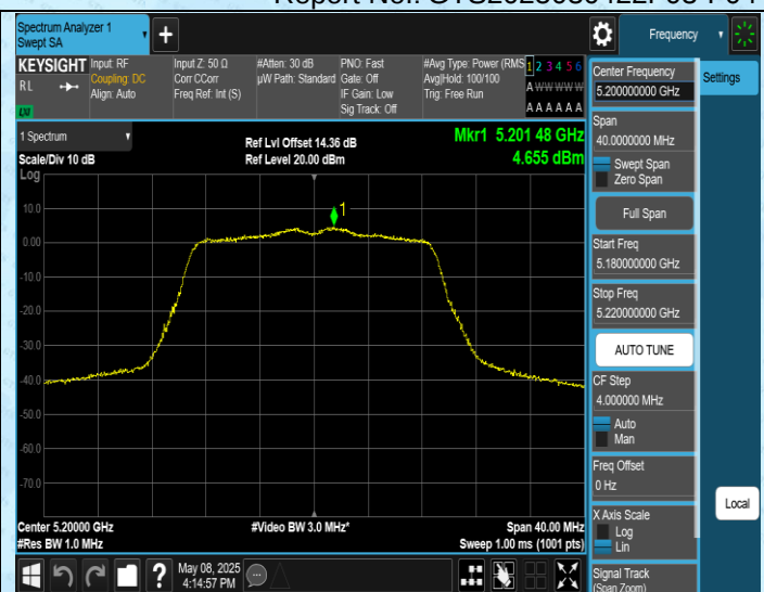
11N20SISO-Ant1-5200-PASS
