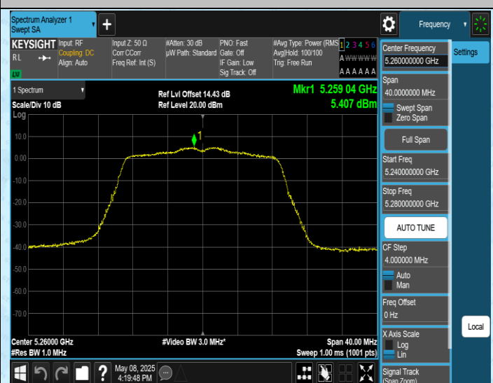
11N20SISO-Ant1-5260-PASS
