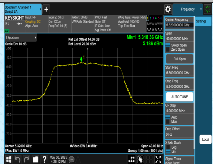
11N20SISO-Ant1-5320-PASS
