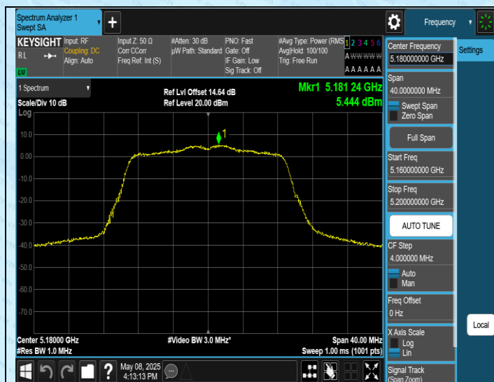
11N20SISO-Ant1-5180-PASS
