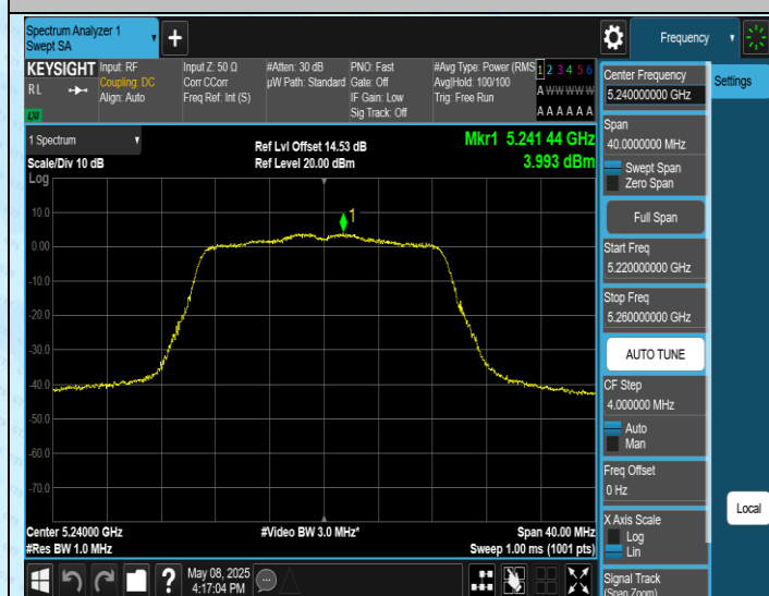
11N20SISO-Ant1-5240-PASS
