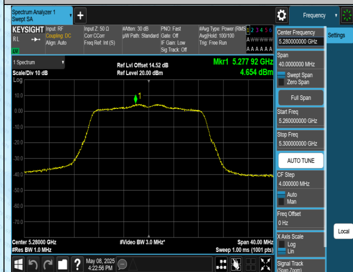
11N20SISO-Ant1-5280-PASS
