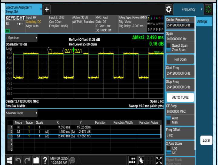
NTNV-11AX20SISO-Ant1-2412
