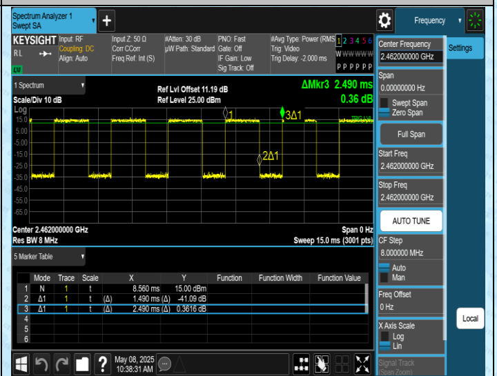
NTNV-11AX20SISO-Ant1-2462
