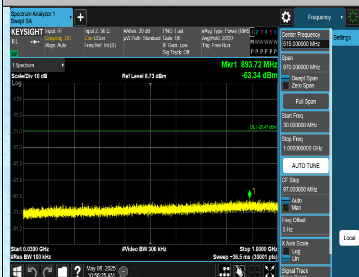
11N20SISO-Ant1-2412-30-1000-PASS
