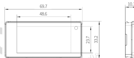
Figure 2-5 2.13" dimension
