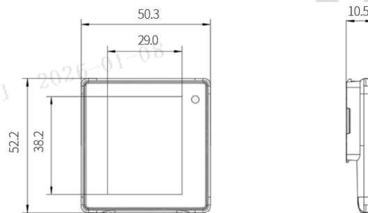
Figure 2-4 2.0" dimension
